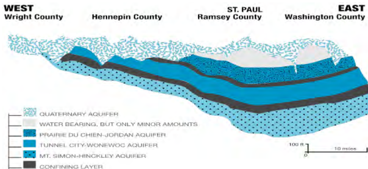
Figure 15. Geologic cross-section of aquifers service the metro area, from east to west across the northern metro.
