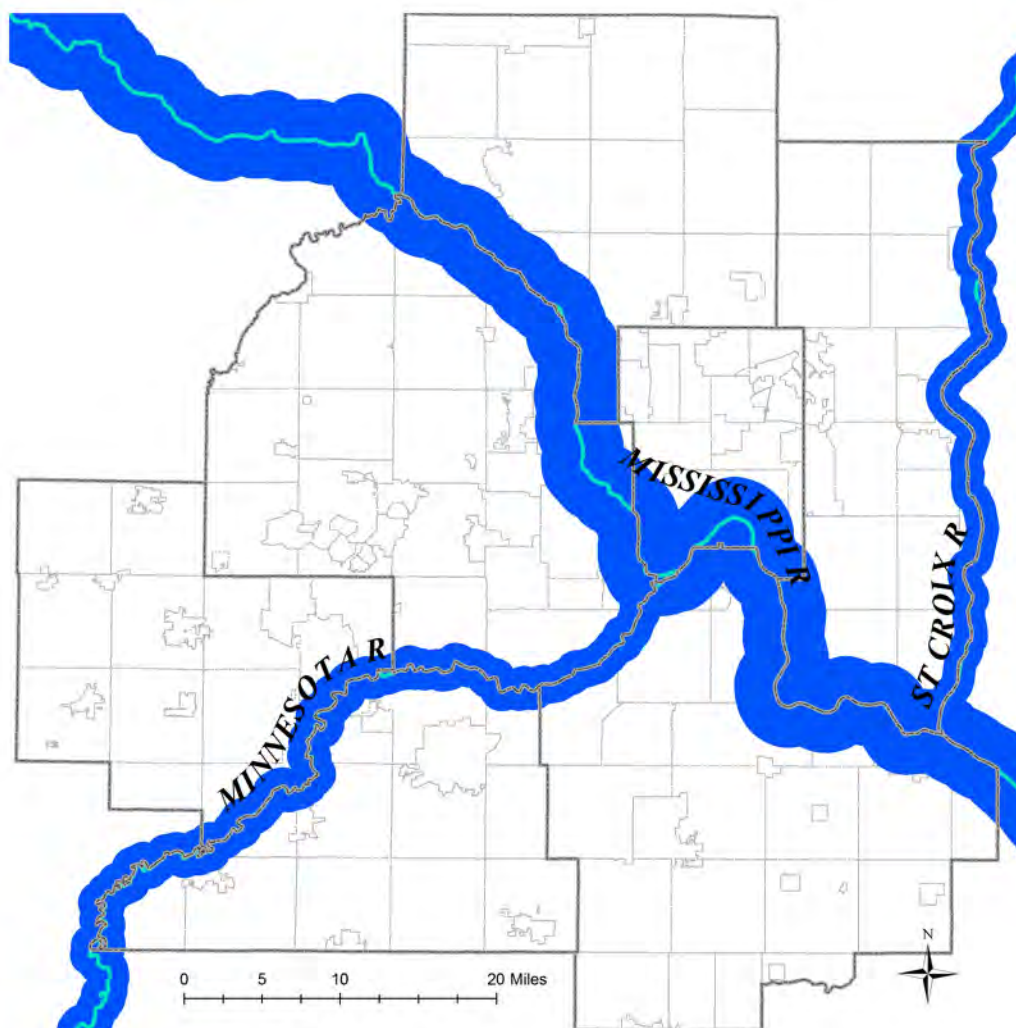
Figure 16. Metro area's three major rivers, sized relative to the amount of flow that is likely to occur at least 90% of the time.
