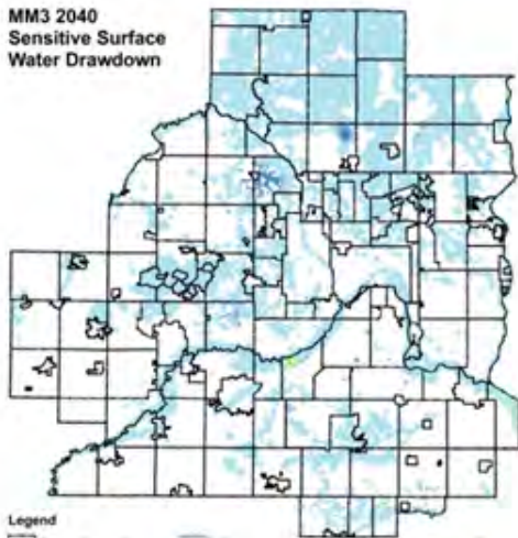
MM3 2040 Sensitive Surface Water Drawdown 20% Increase
