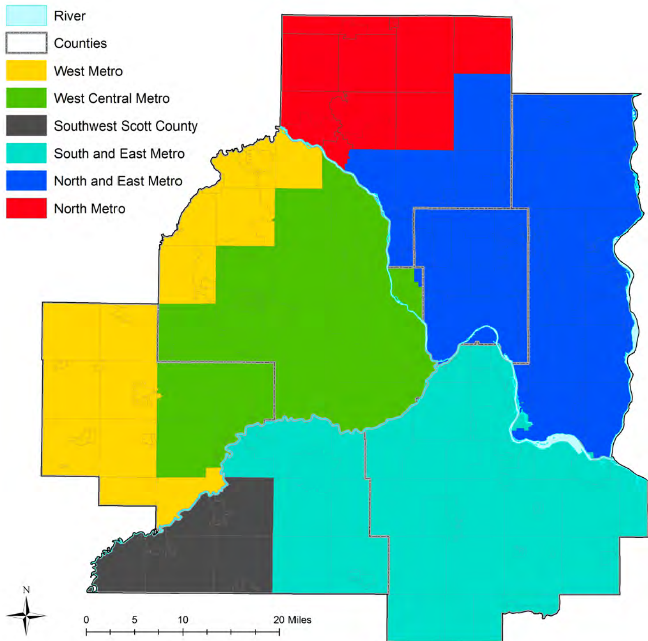
Figure 28. Map of hydrogeologic subregions.
