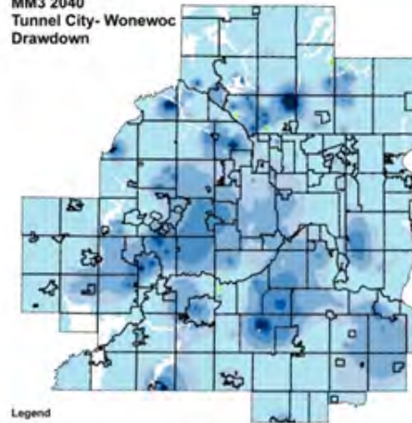
MM3 2040 Tunnel City Wonewoc Drawdown 20% Decrease
