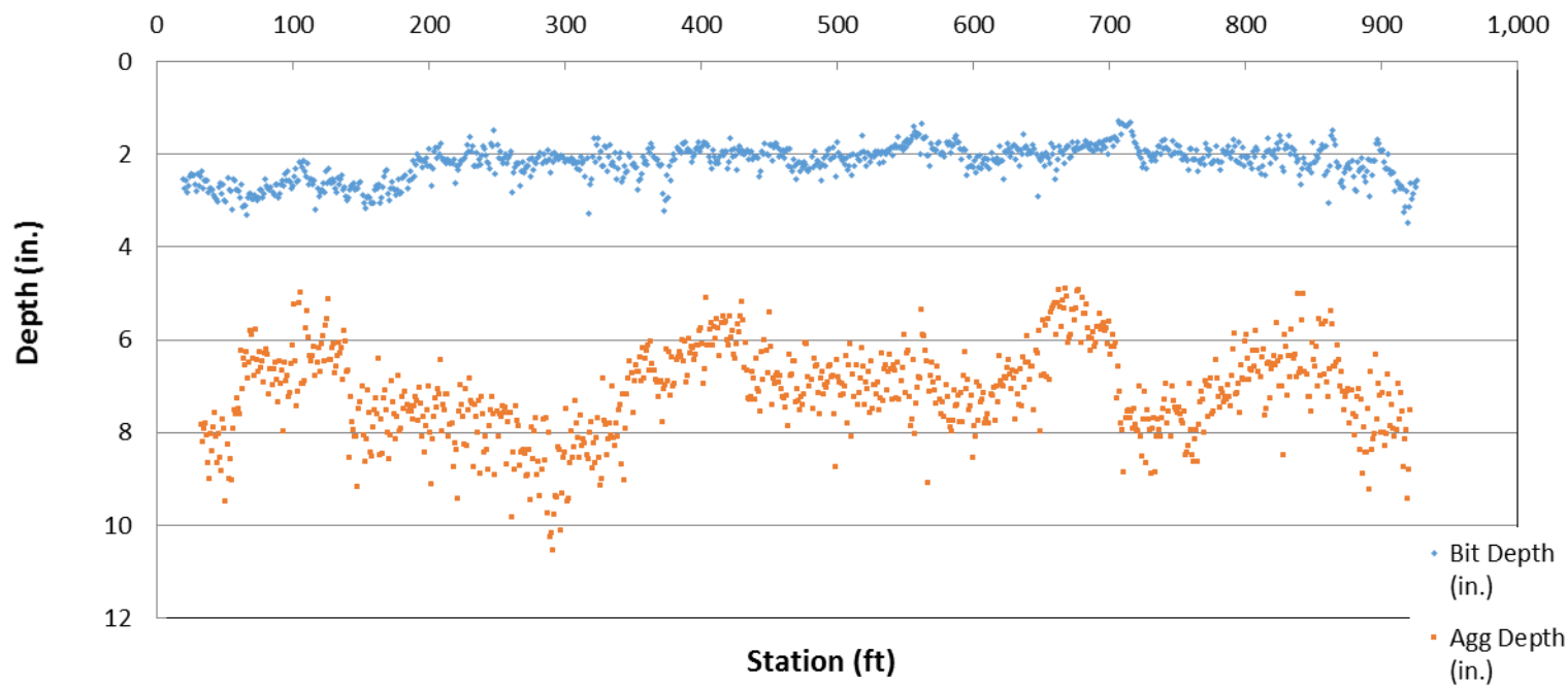
GPR Data Points (163rd Lane: CSAH 83 to Alpaca Street)
