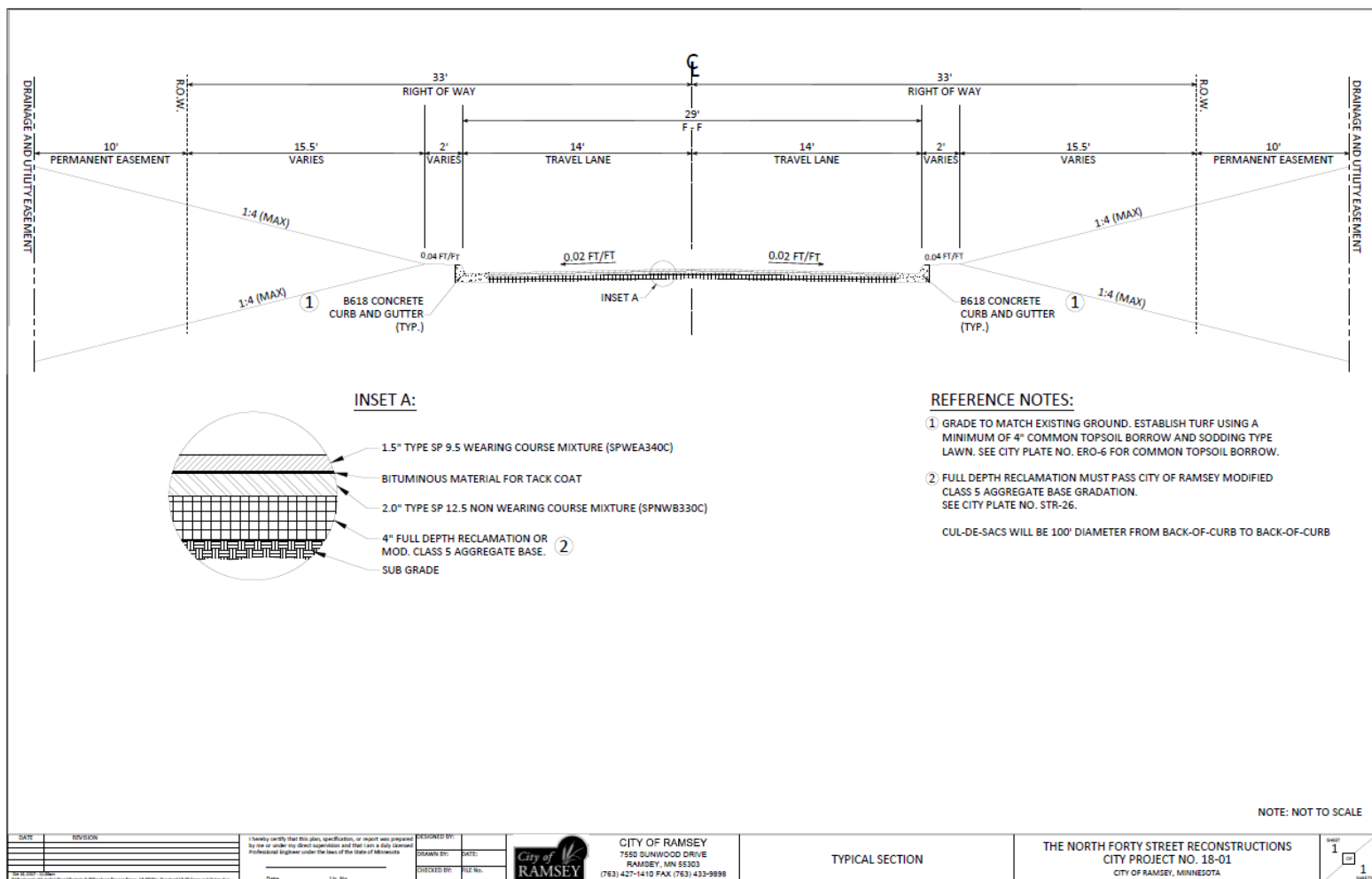
FIGURE 2 TYPICAL SECTION – PROPOSED IMPROVEMENTS
