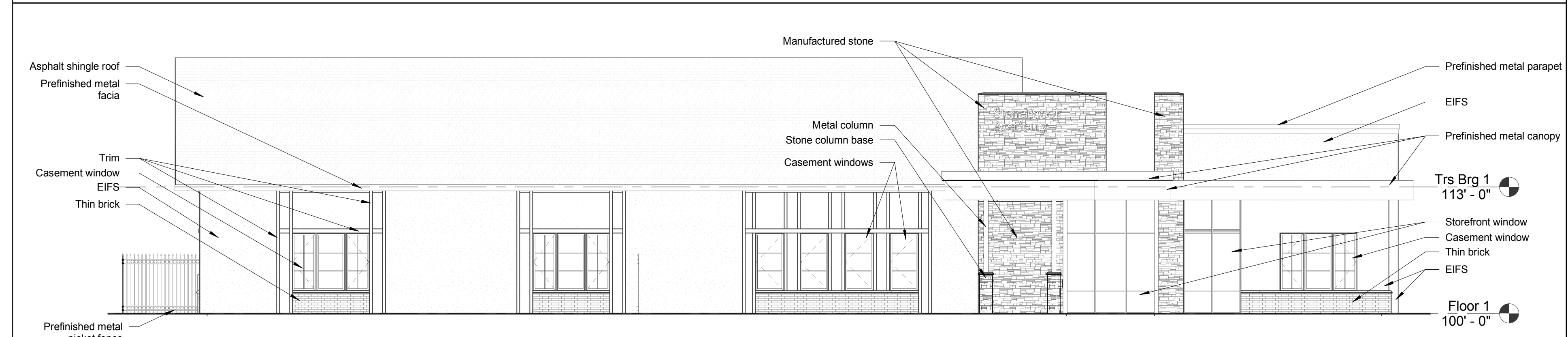
G6 Preliminary South Elevation (View from Veterans Drive) CS02 1/8" = 1'-0"
