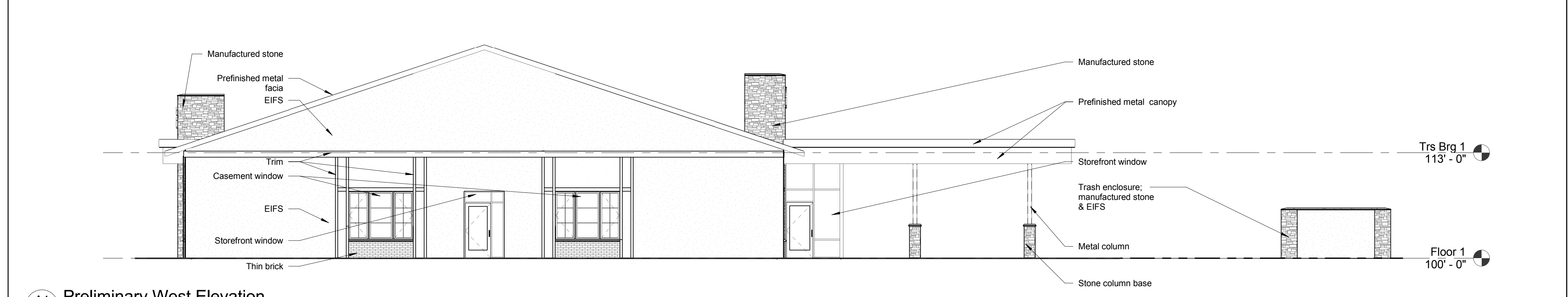
A4 Preliminary West Elevation CS02 1/8" = 1'-0"
