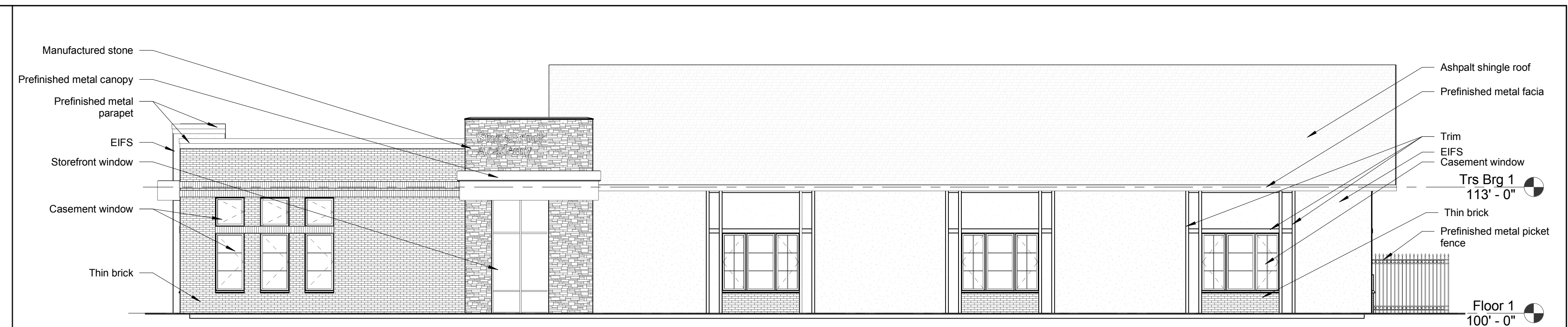
K6 Preliminary North Elevation (View from Sunwood Drive) CS02 1/8" = 1'-0"
