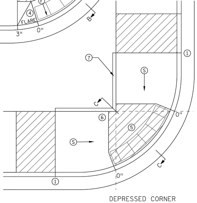
DEPRESSED CORNER
