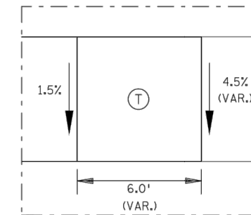
INSET A TRANSITION PANEL (4,5)
