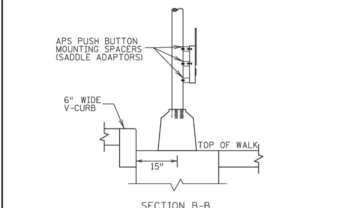
SIGNAL PEDESTAL & PUSH BUTTON (V-CURB)
