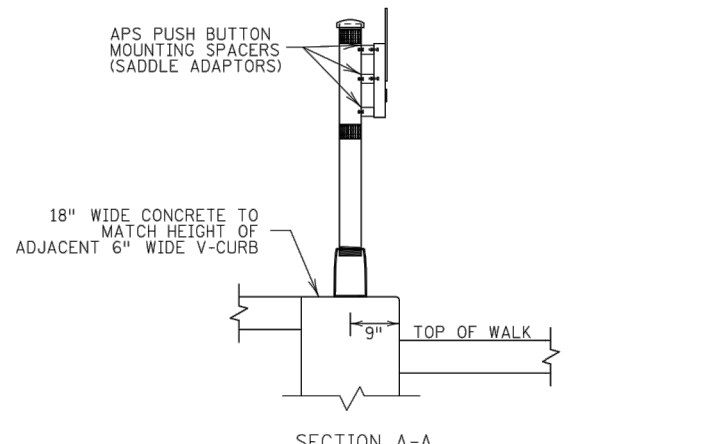
PUSH BUTTON STATION (V-CURB)
