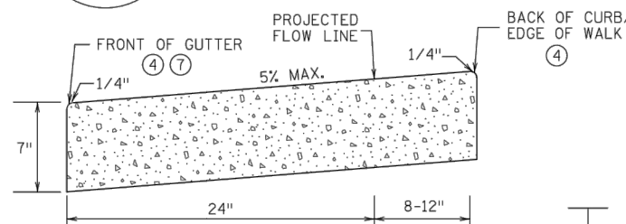
INSET B OUTFLOW GUTTER ⑧
