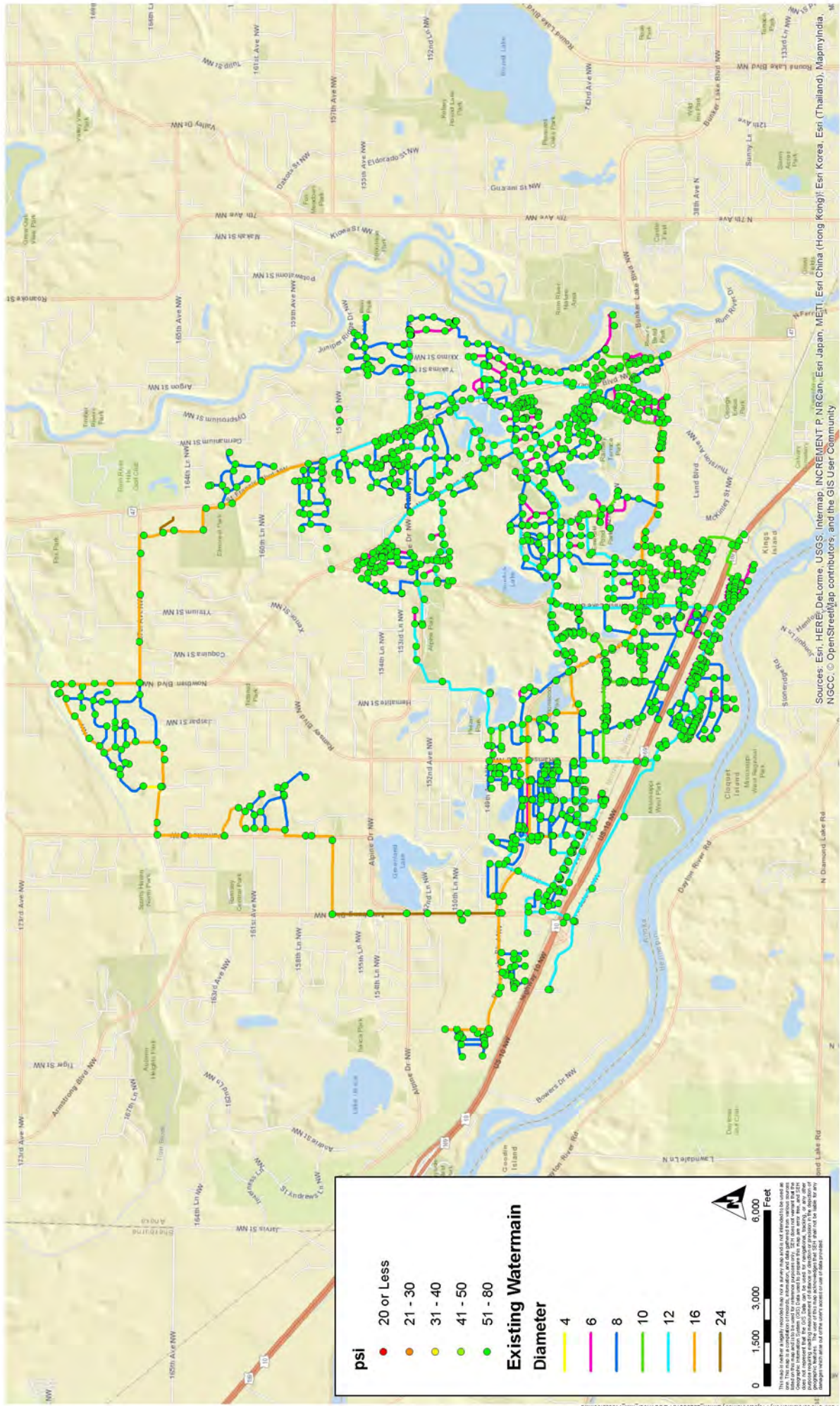
FIGURE 6 Minimum Pressures
