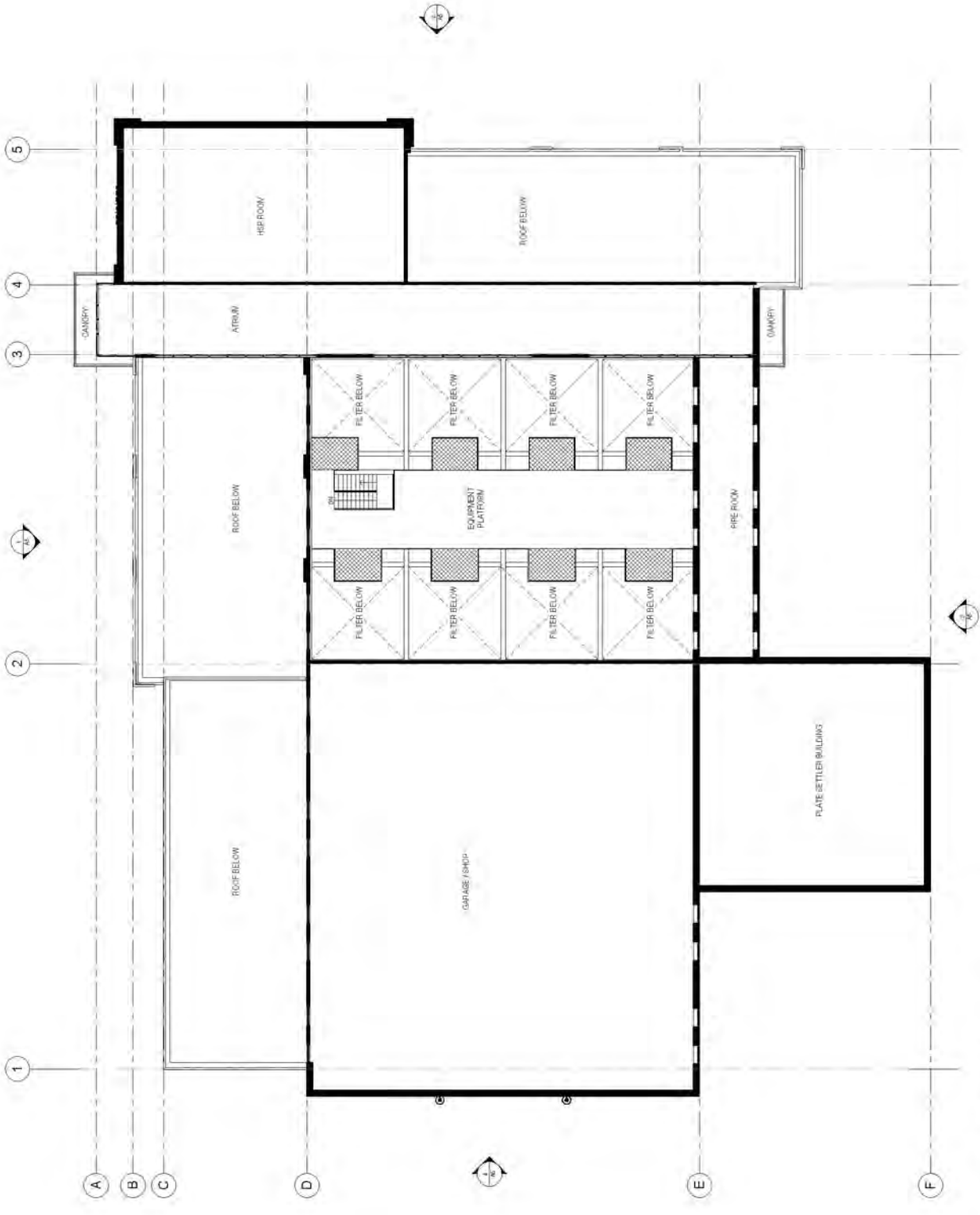
UPPER LEVEL FLOOR PLAN - ALTERNATIVE 1
