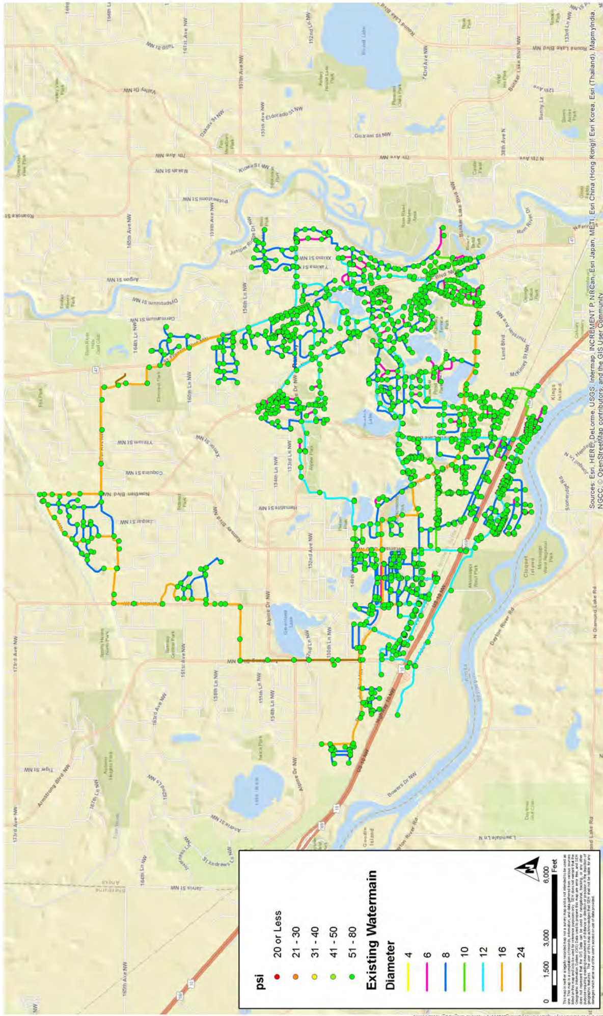
FIGURE 12 Minimum Pressures
