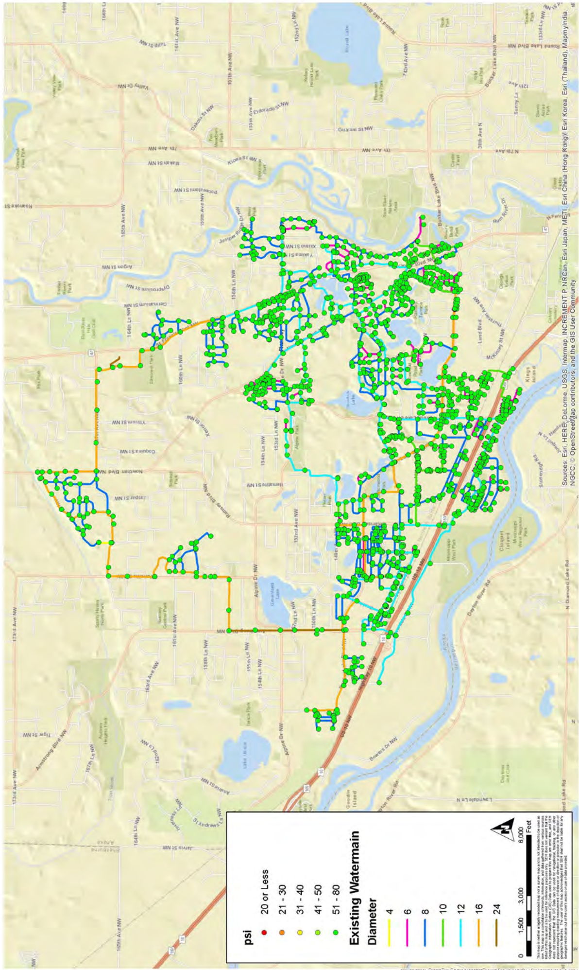
EXISTING MDD STATIC PRESSURE Ramsey, Minnesota
