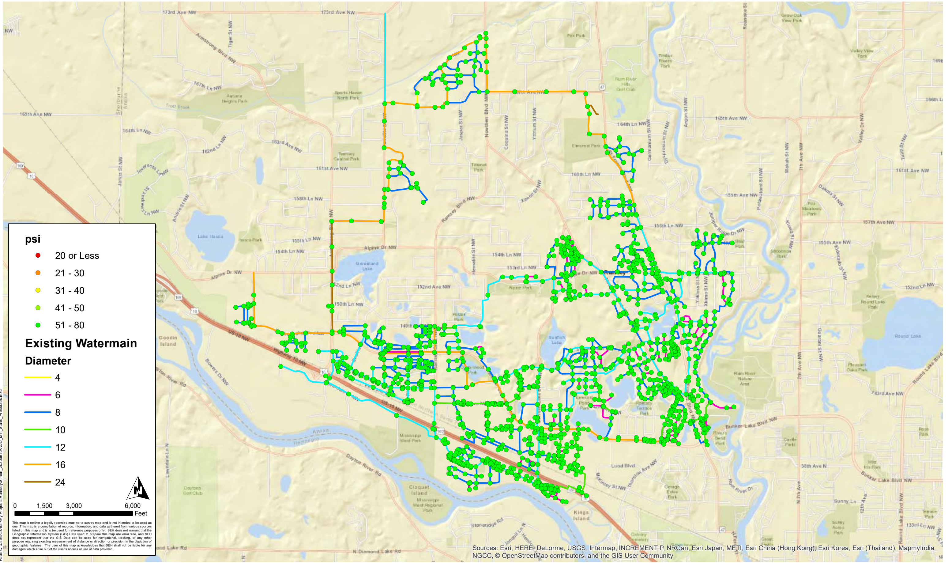
FIGURE 1 Minimum Pressures
