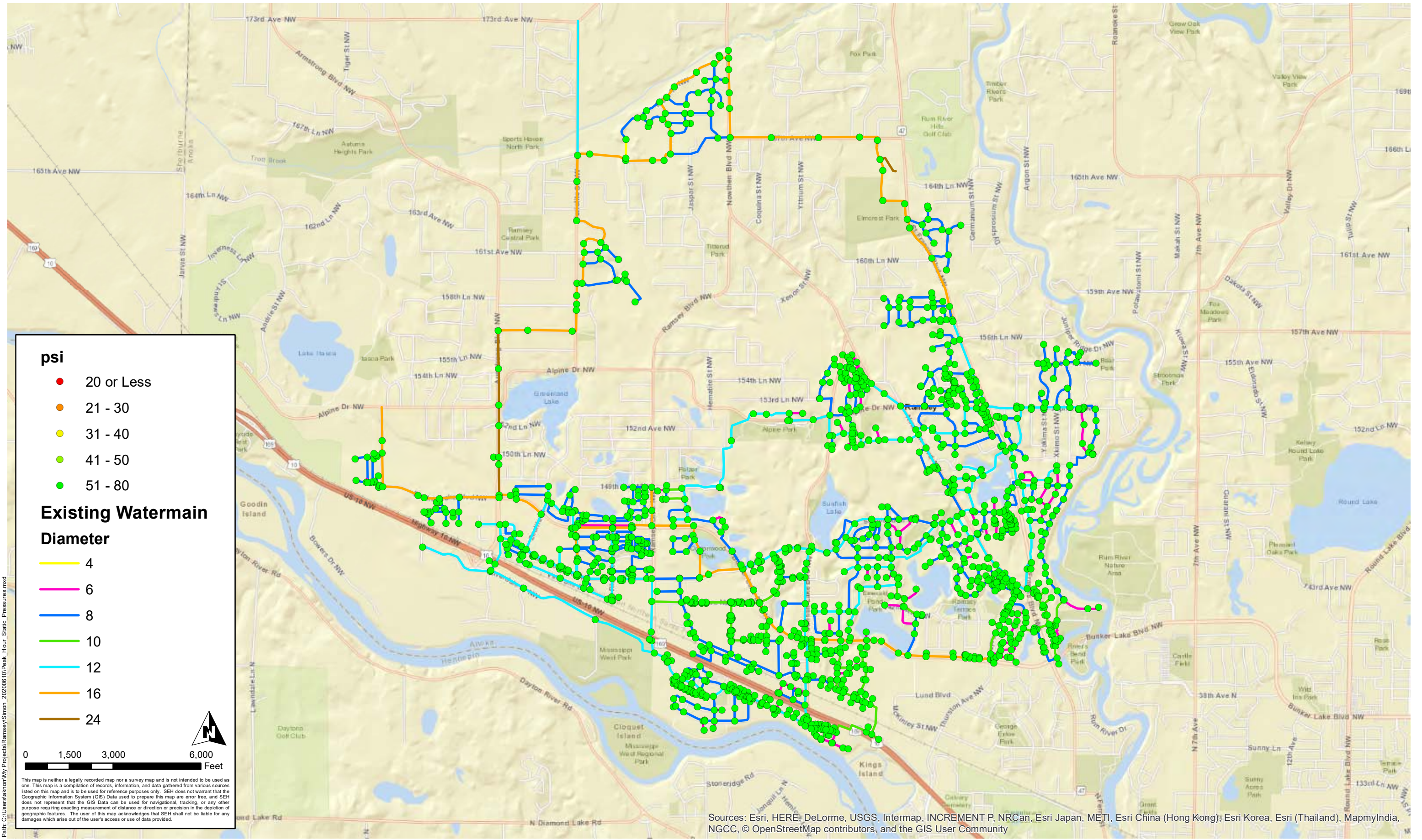
FIGURE 3 Minimum Pressures
