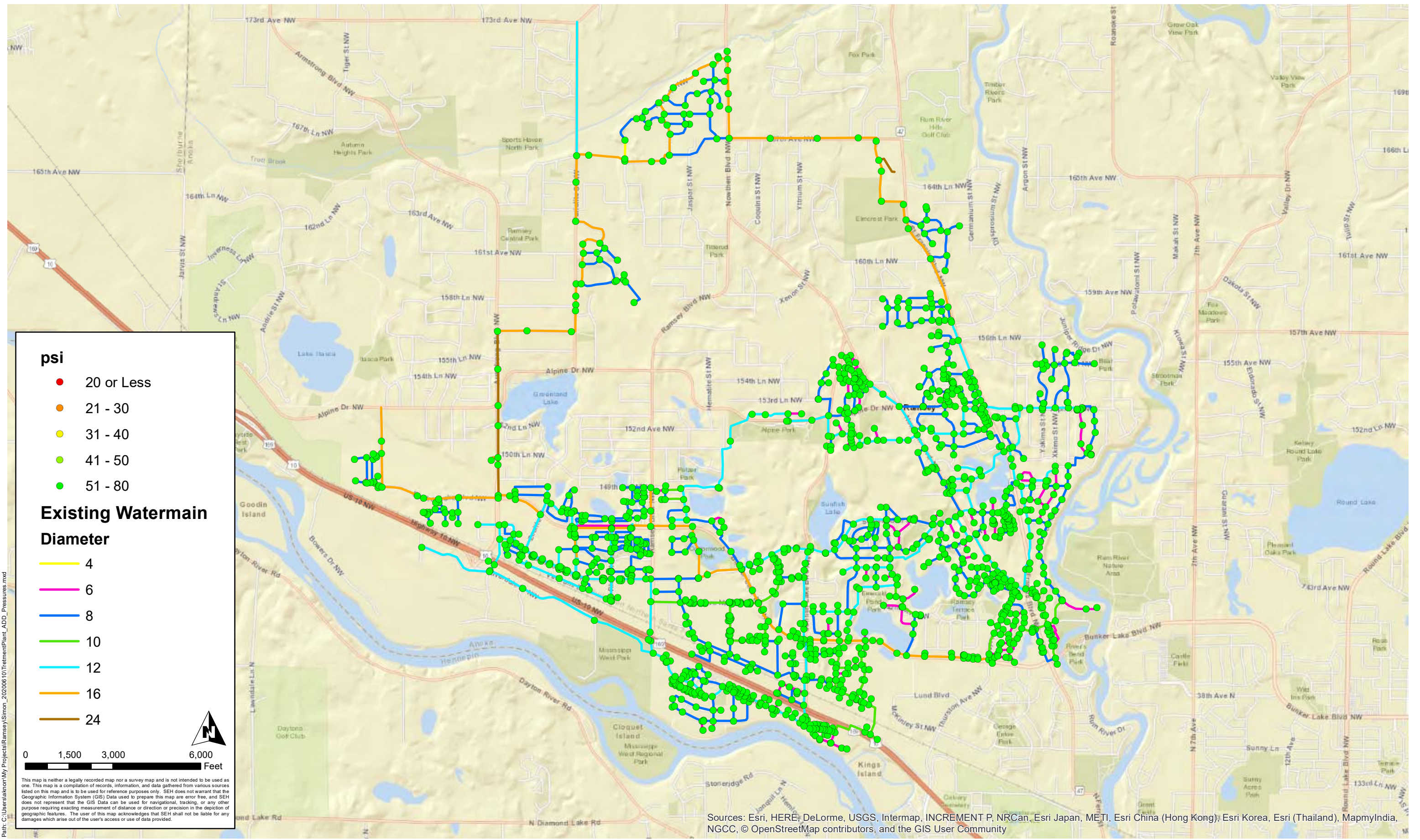
FIGURE 11 Minimum Pressures
