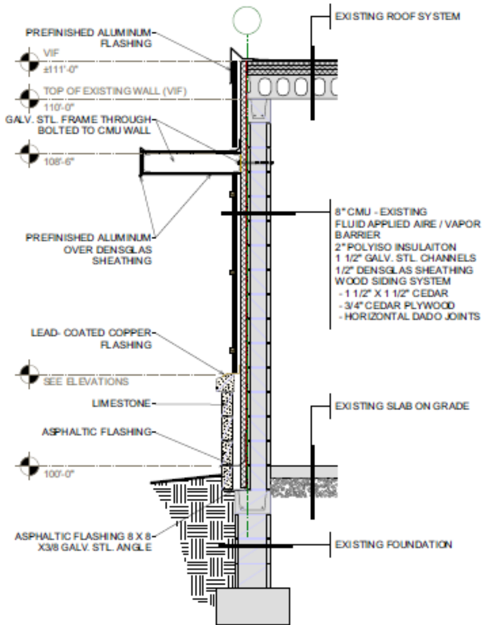
1 TYPICAL WALL SECTION AS.1 Scale: 1/2" = 1'-0"
