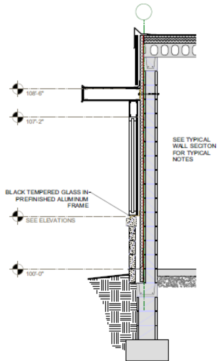
2 WALL SECTION AT ALUMINUM PANEL AS.1 Scale: 1/2" = 1'-0"
