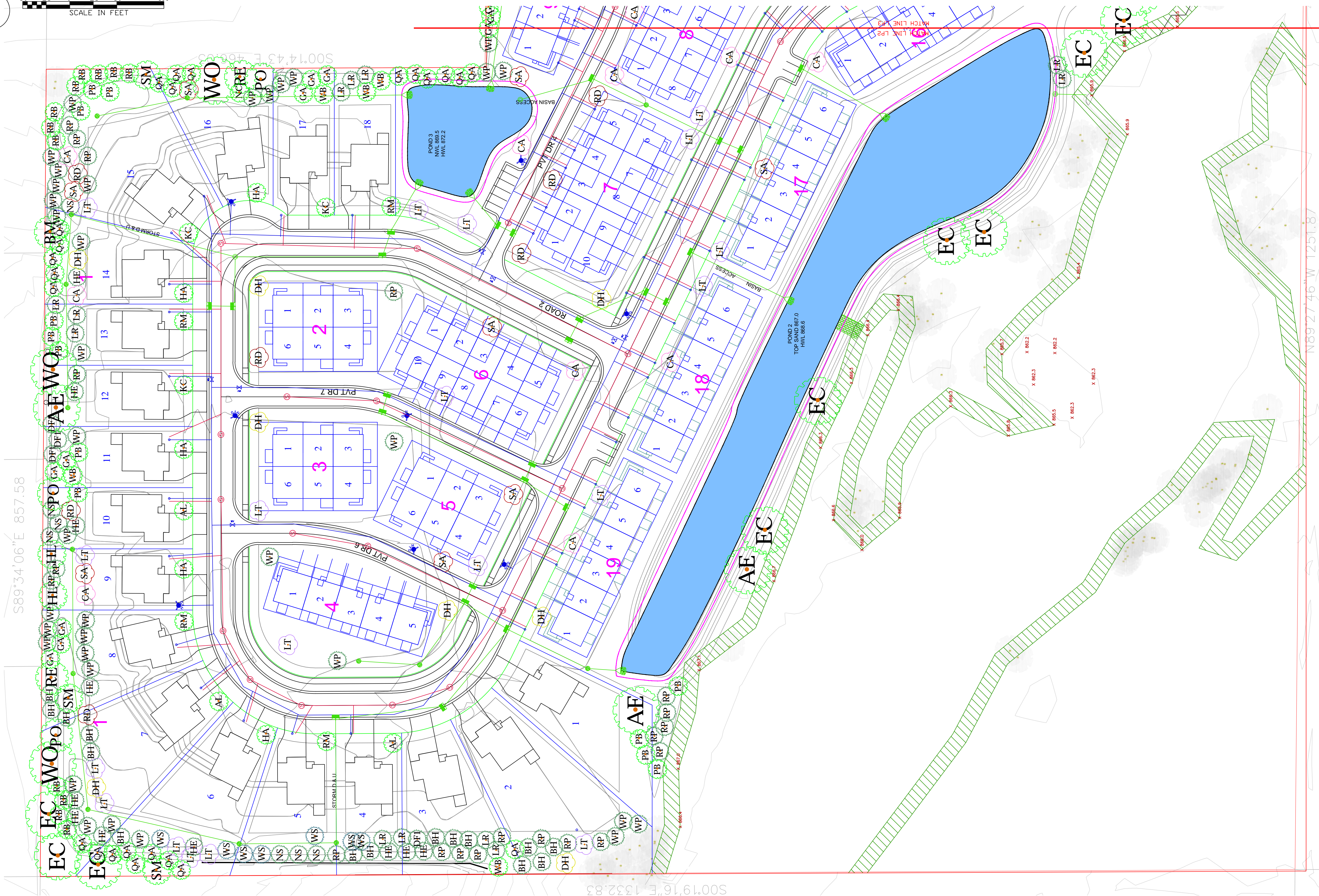
2 Planting Plan 1 SCALE: 1" = 50'
