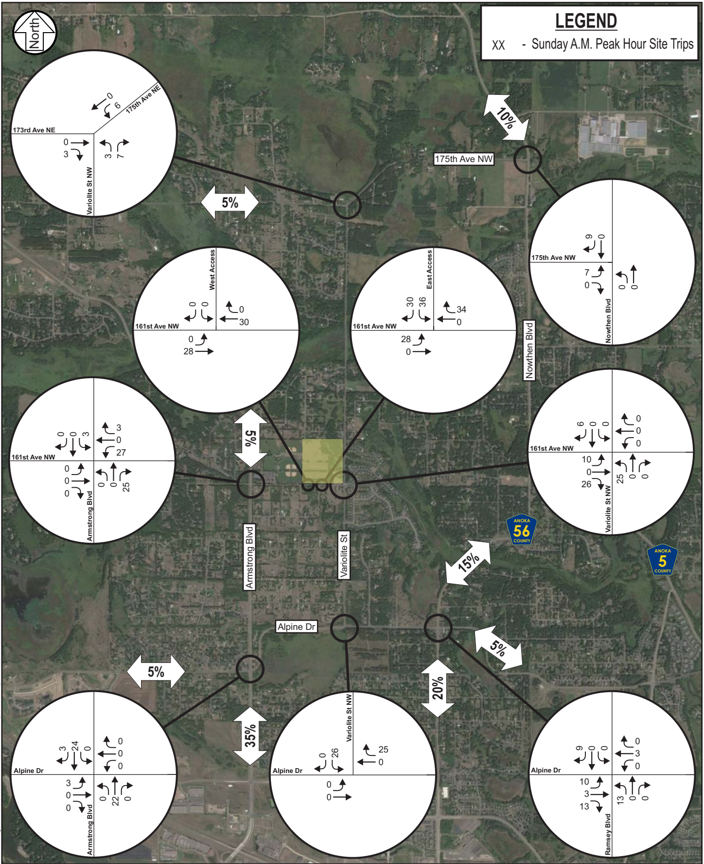
Peak Hour Site Generated Trip Directional Distribution - Sunday PACT Charter School Traffic Impact Study Ramsey, MN
