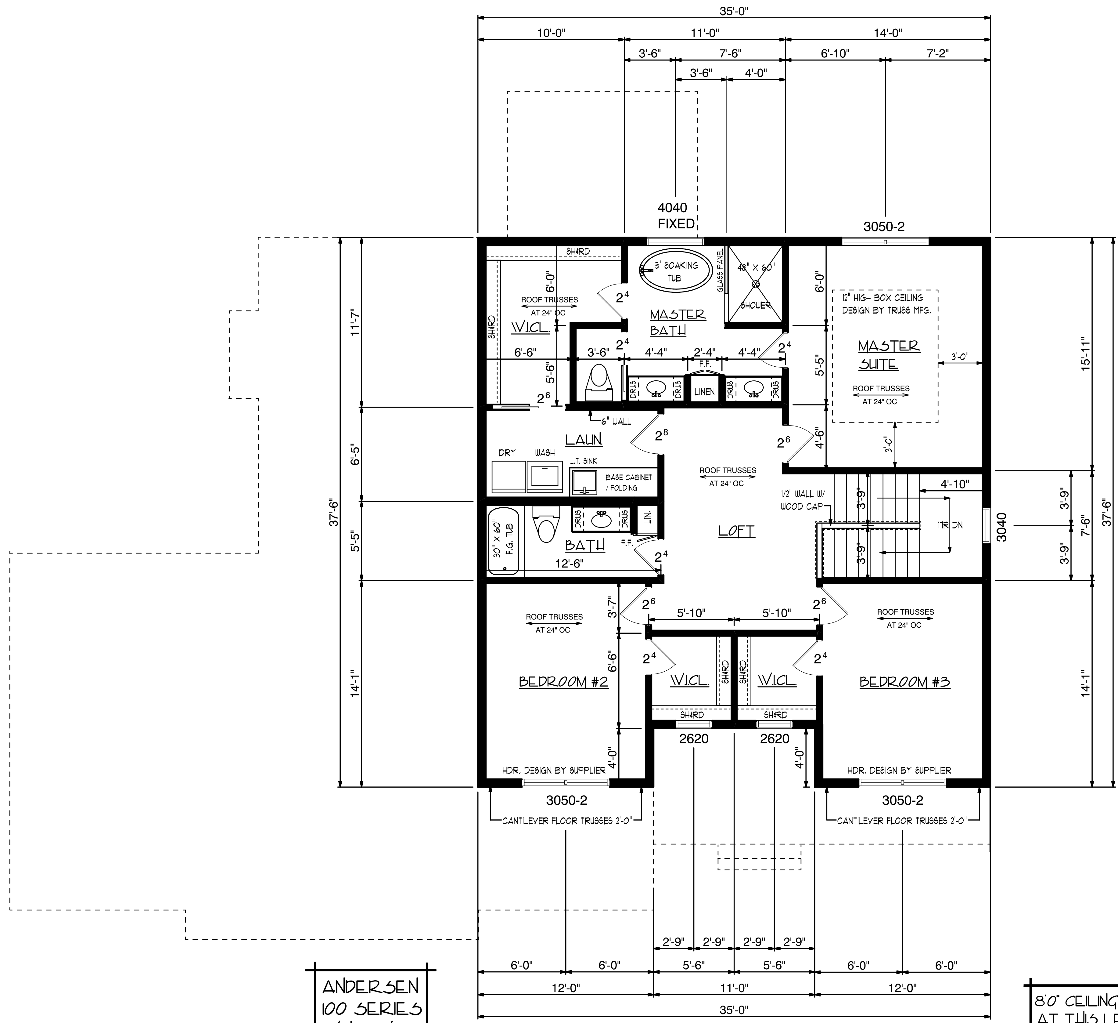
UPPER FLOOR PLAN 1/4" STREICH CUSTOM HOME DESIGN 1268 SQ. FT.
