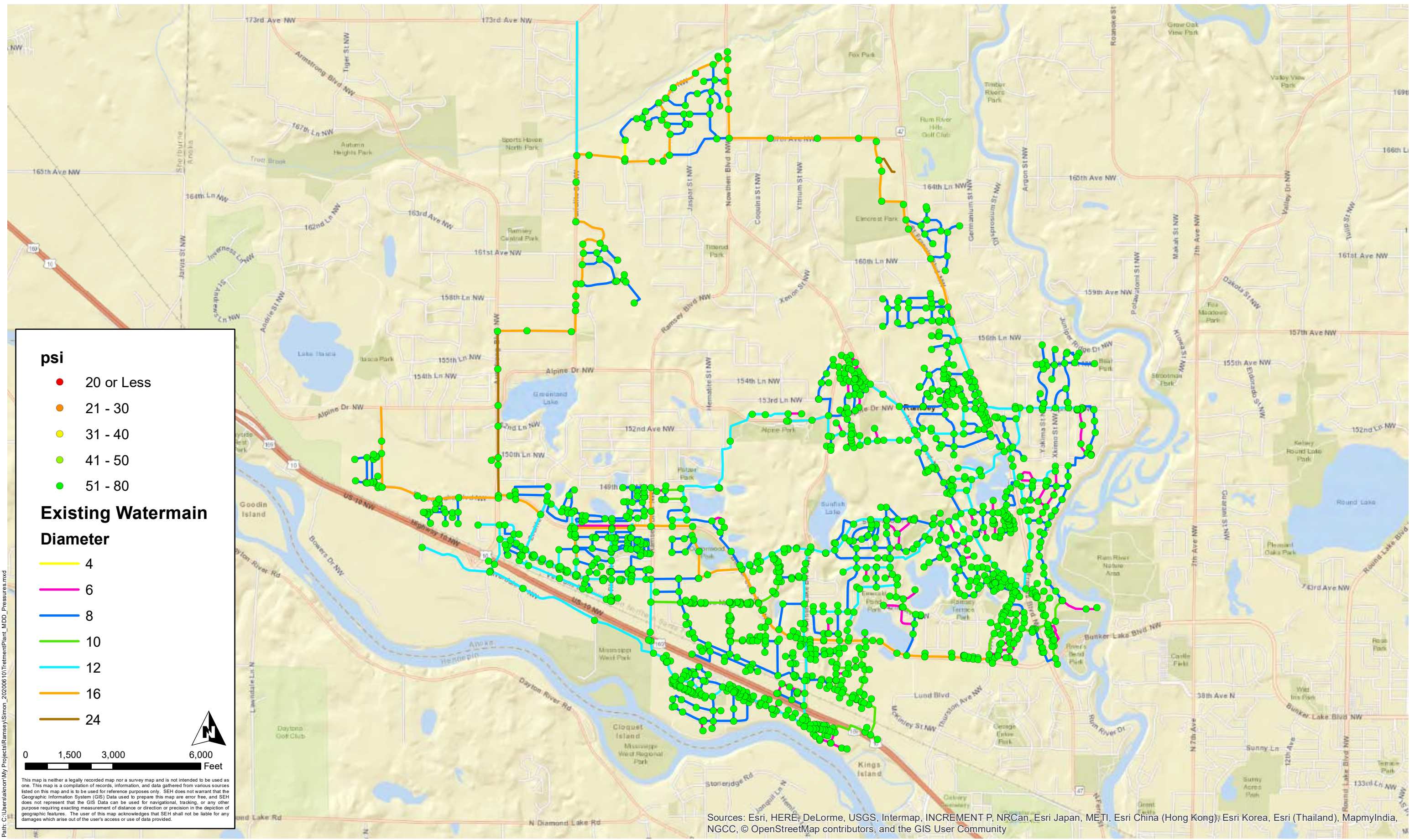
FIGURE 12 Minimum Pressures
