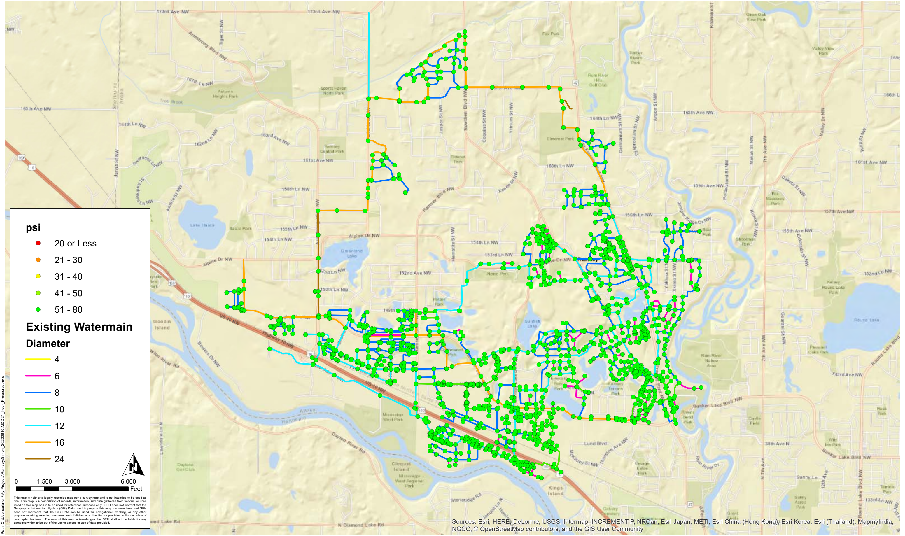
FIGURE 7 Minimum Pressures
