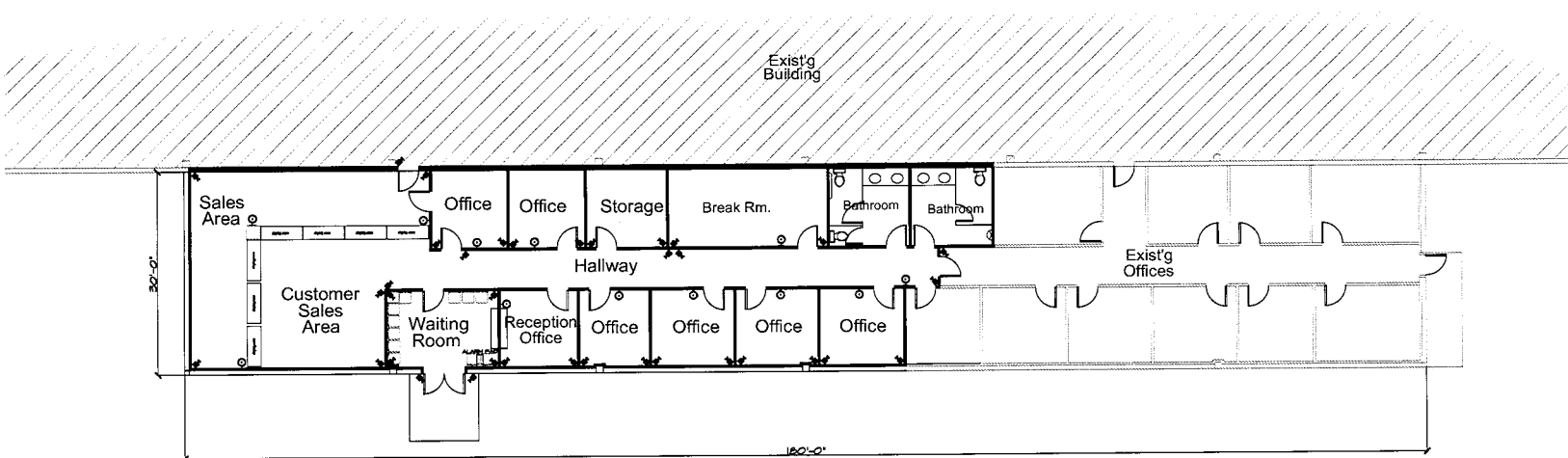
(NEW) DISPENSARY FLOOR PLAN SCALE: 1/8" = 1'-0"
