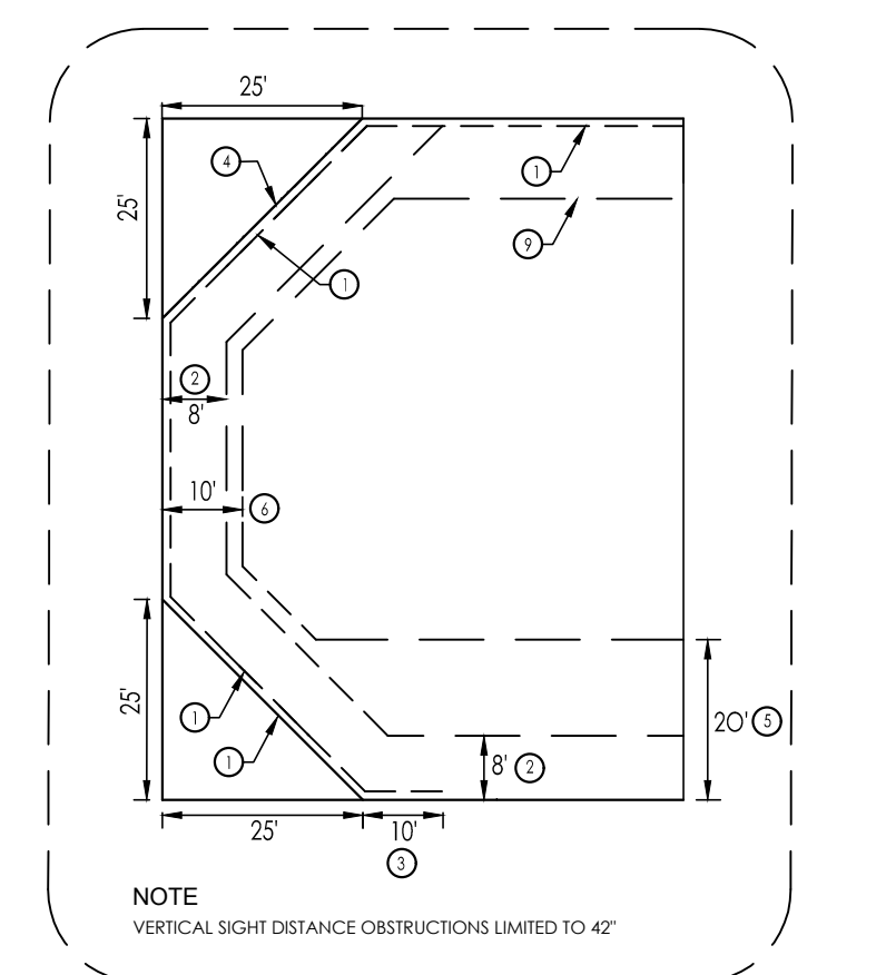
TYPICAL CORNER LOT DETAIL
