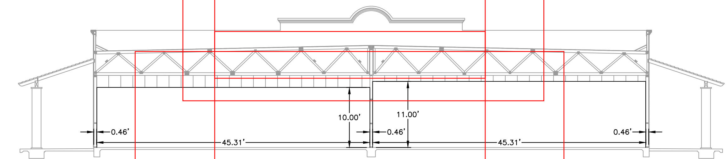
SUITE A BUILDING SECTION
