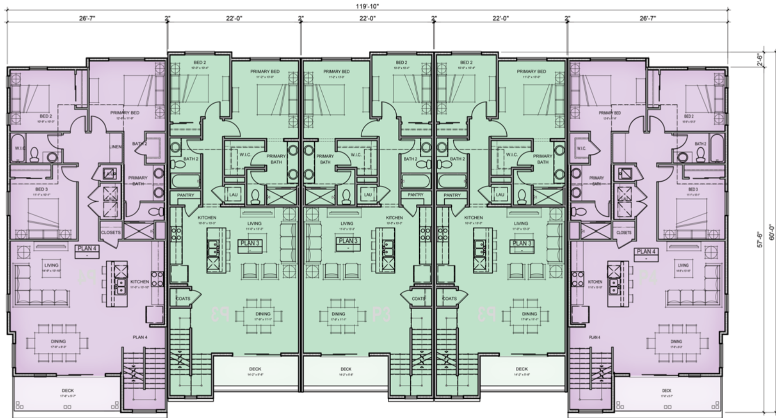
THIRD FLOOR
