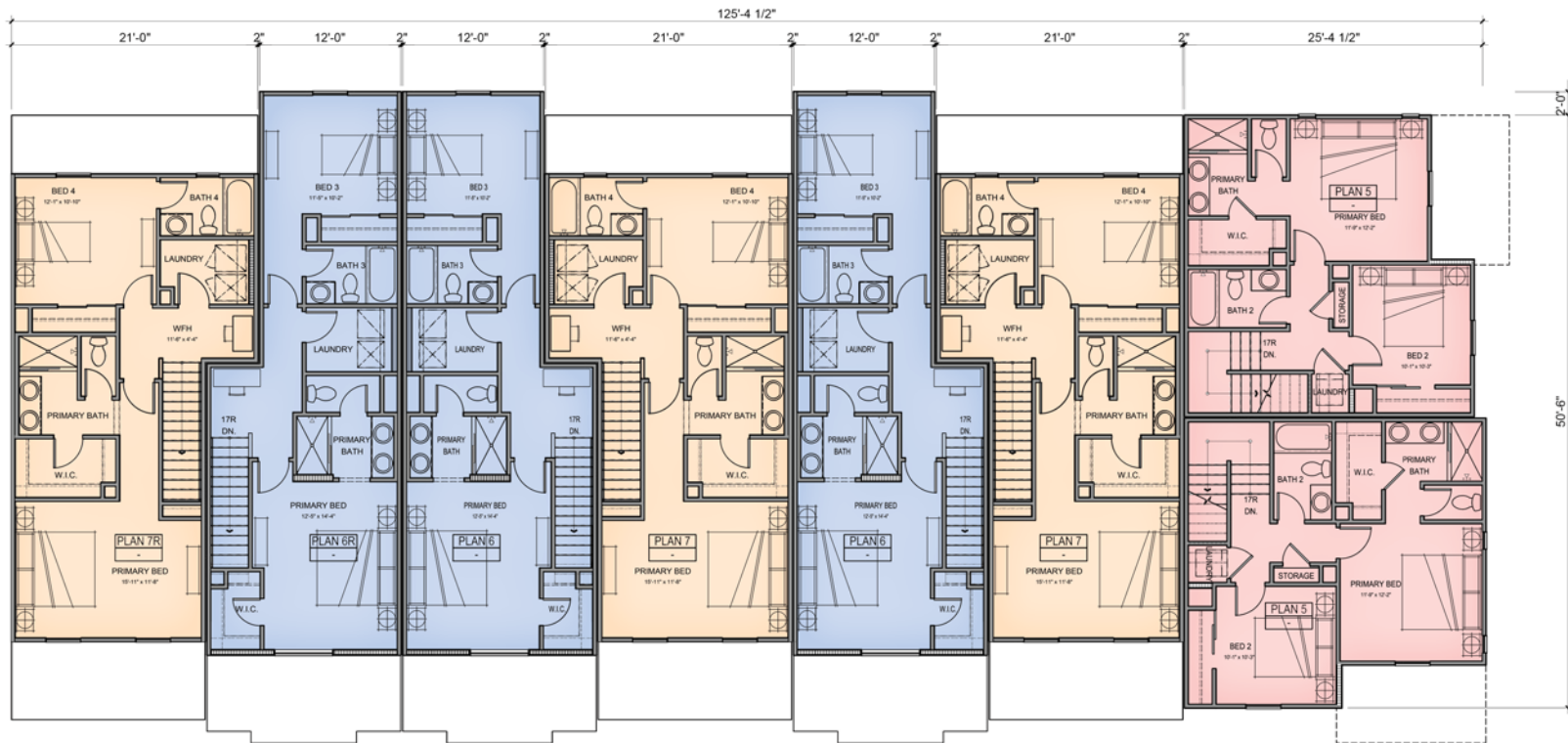
THIRD FLOOR
