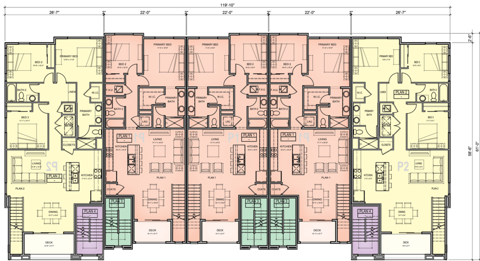
SECOND FLOOR
