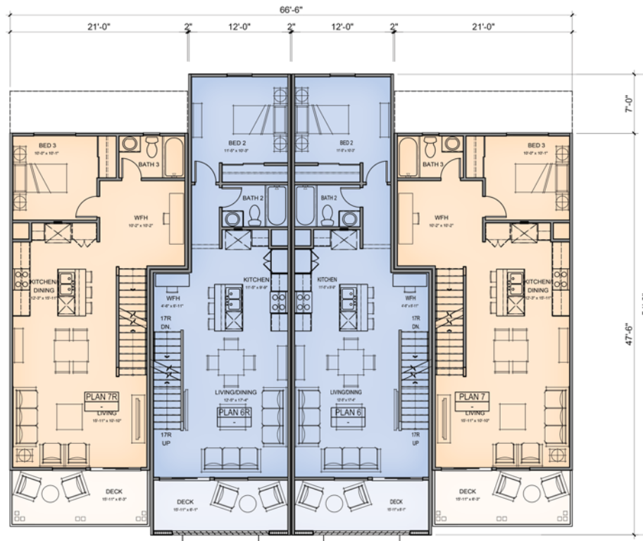
SECOND FLOOR
