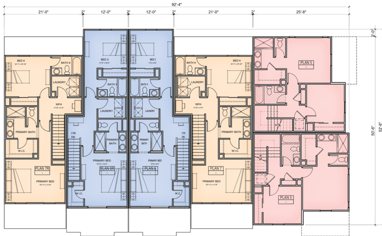
THIRD FLOOR
