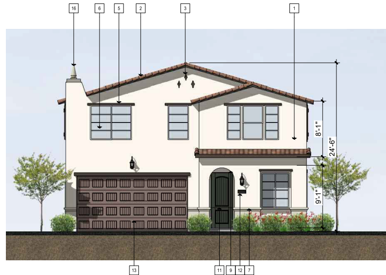
Exhibit 3.3b: Plan 3522 Elevations
