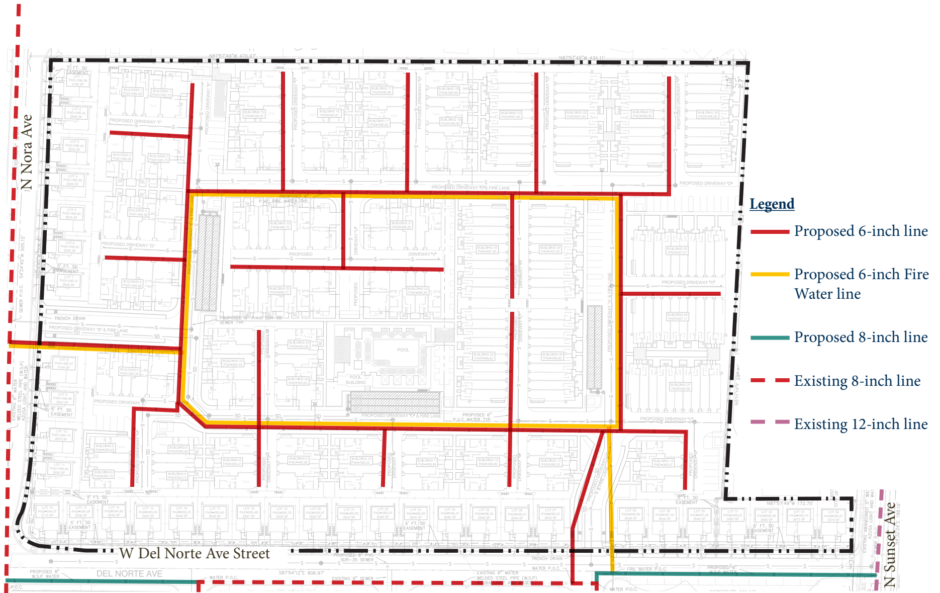
Exhibit 5.4: Conceptual Domestic Water Plan
