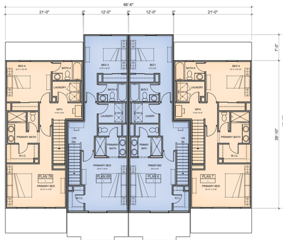
THIRD FLOOR
