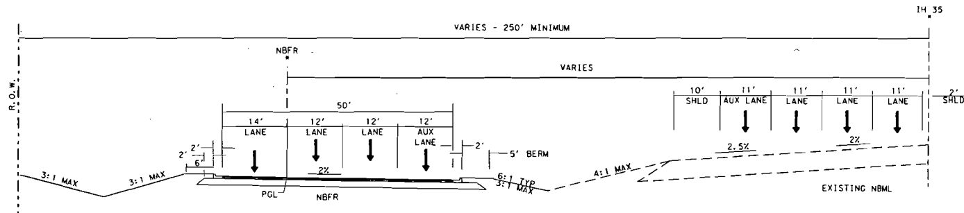
PROPOSED IH 35 NBFR (3 LANES W/ AUX)
