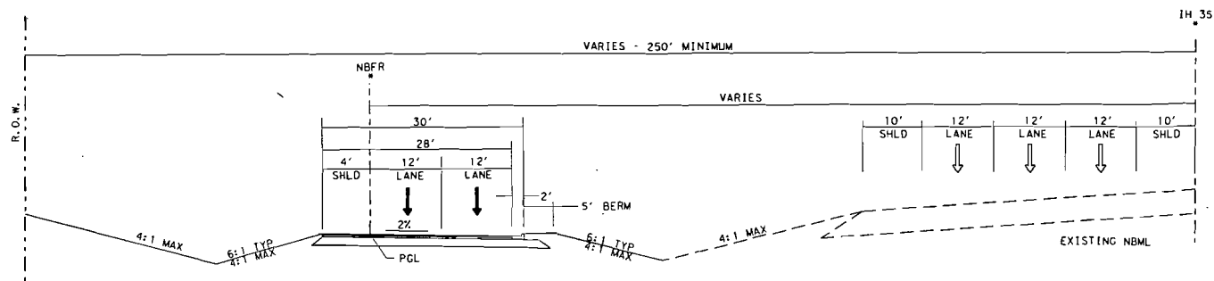
PROPOSED IH 35 NBFR (2 LANES W/O AUX)
