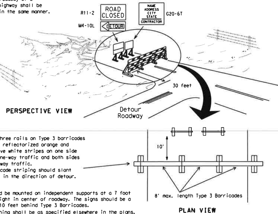
TYPE 3 BARRICADE (POST AND SKID) TYPICAL APPLICATION
