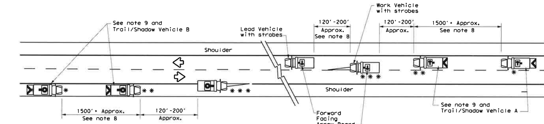
TCP (3-1b) TWO-WAY ROADWAY WITH PAVED SHOULDERS
