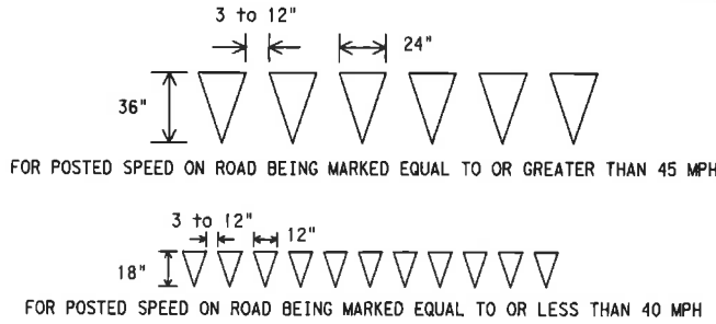
YIELD LINES
