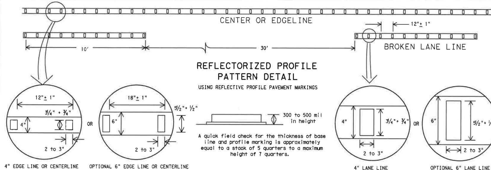
DETAIL "A"
