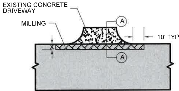
CONCRETE DRIVEWAY TYPICAL X = 5'
