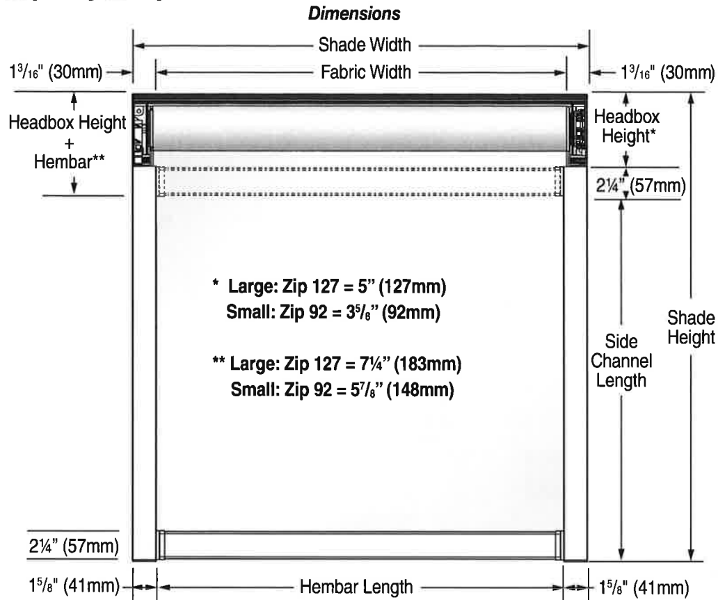
Side Channel Dimensions
