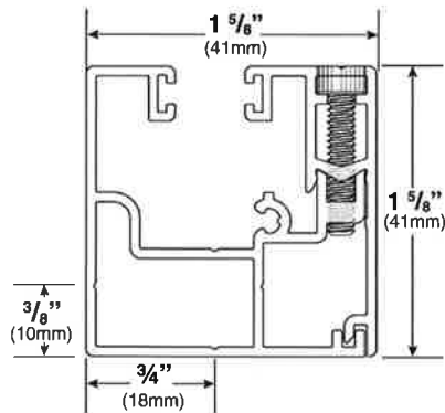
Zip 92 Mounting Bracket
