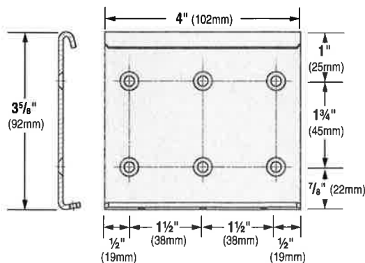
Zip 92 Mounting Bracket
