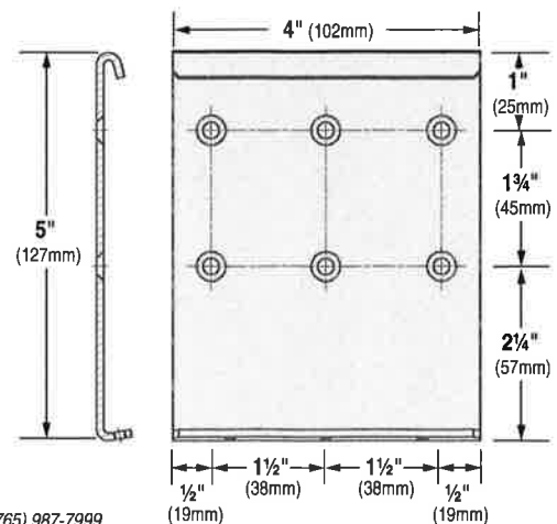
Zip 127 Mounting Bracket
