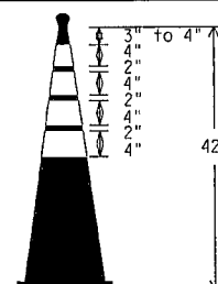
EDGELINE CHANNELIZER
