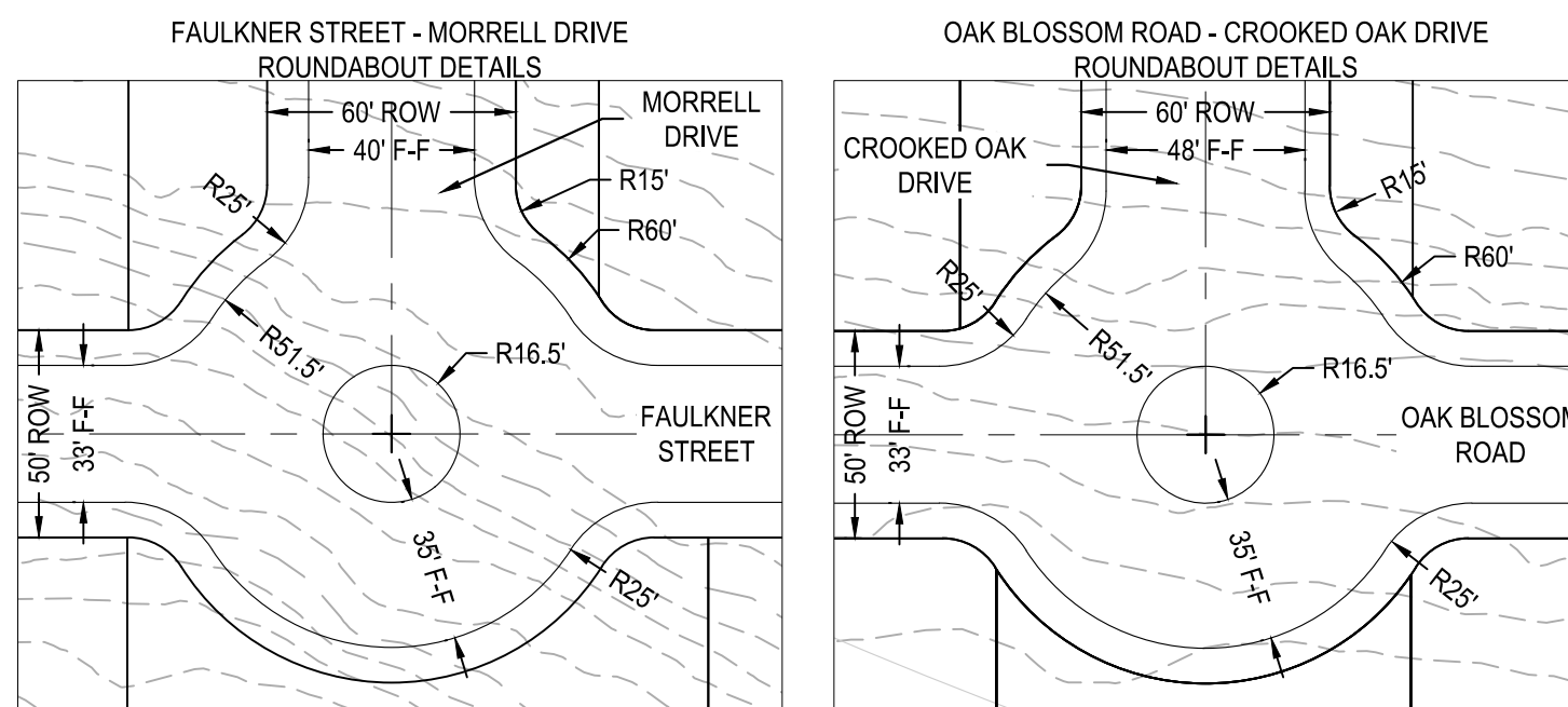
TYPICAL UTILITY ASSIGNMENT DETAIL N.T.S.
