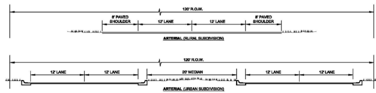
TYPICAL ARTERIAL SECTION
