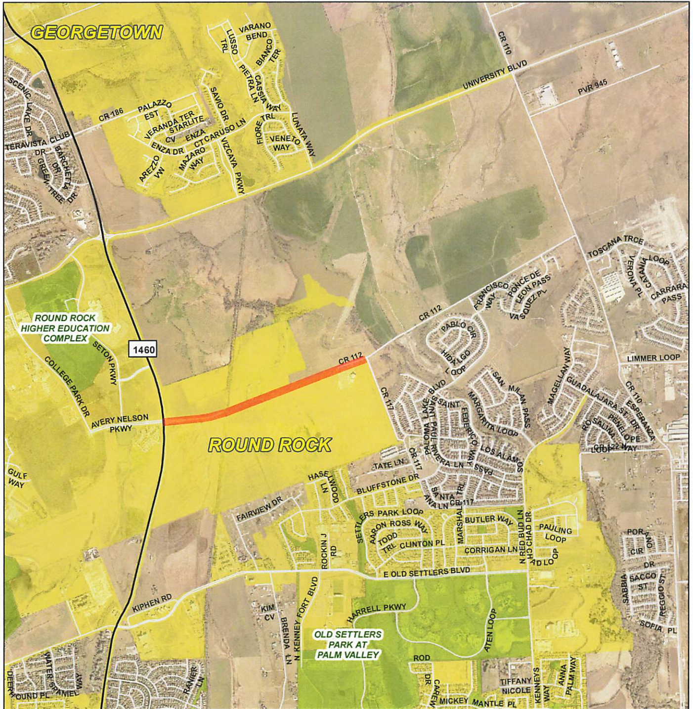
Exhibit A: Location of CR 112 Widening (FM 160 / AW Grimes to CR 117)
