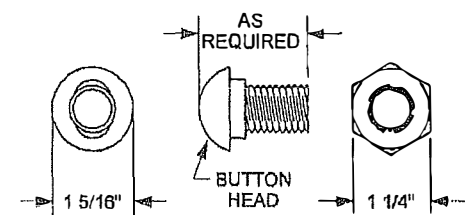
5/16" POST OR SPLICE BOLT OVAL SHOULDER SHALL BE OF ADEQUATE HEIGHT, LENGTH & SHAPE TO PREVENT TURNING DURING INSTALLATION OR REMOVAL OF BOLT.
