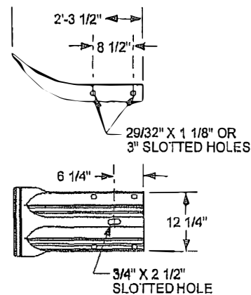
12 GAGE END SECTION
