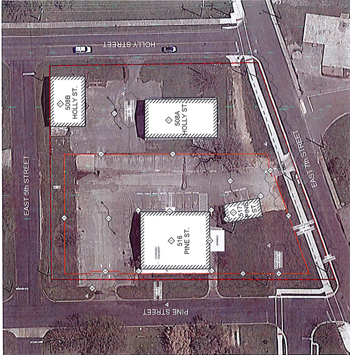
1 SITE PLAN 1" = 20'-0"
