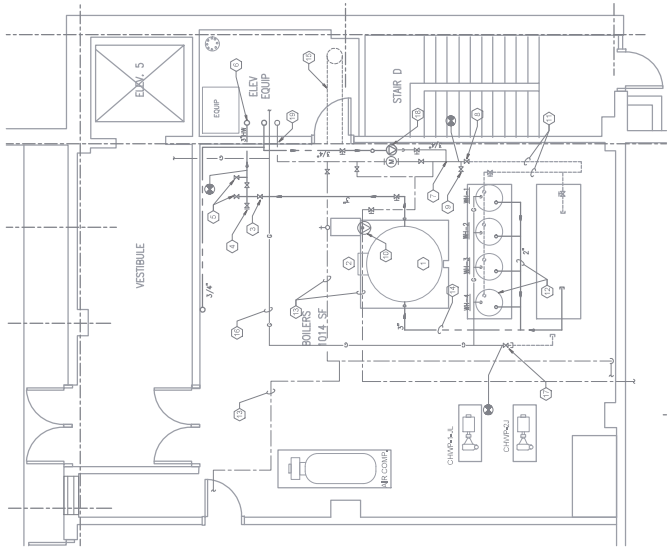
1 BOILER ROOM - DEMO & PREP
