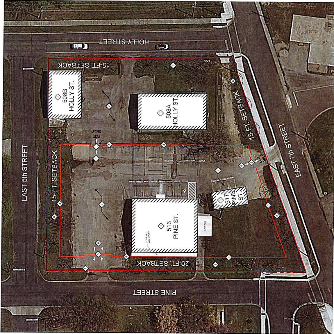
1 SITE PLAN 1" = 20'-0"
