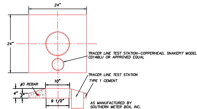
CONCRETE PAD
