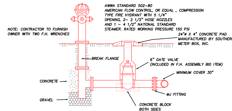
6" FIRE HYDRANT ASSEMBLY
