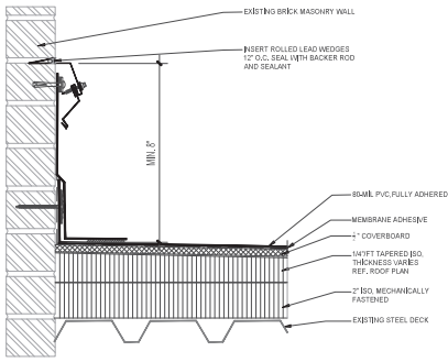
1 SECTION C ROOF TO BRICK RISE WALL SCALE: 3/4"=1'-0"
