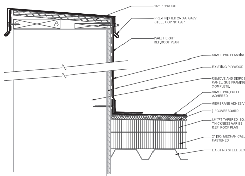
2 SECTION B WALL PANEL MODIFICATION SCALE: 3/4"=1'-0"
