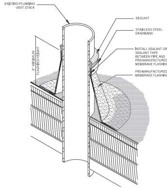
2 PRE-MFD PLUMBING VENT FLASHING SCALE: 3/4" = 1'
