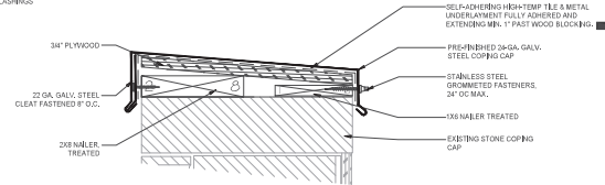
3 COPING CAP @ EXISTING STONE SCALE: 3/4"=1'-0"
