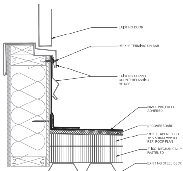
4 DOOR THRESHOLD SCALE: NTS
