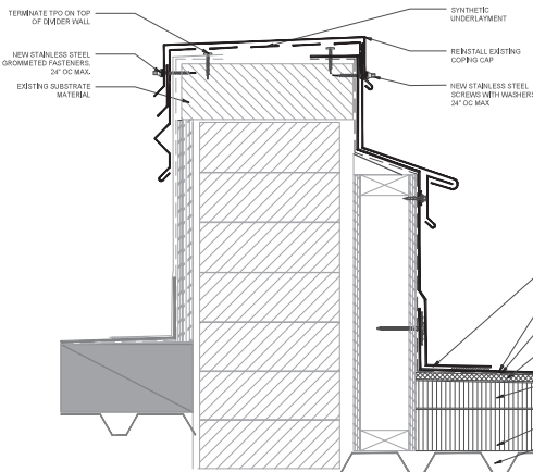
2 SOUTH ROOF EJ SCALE: 5/8"=1'-0"
