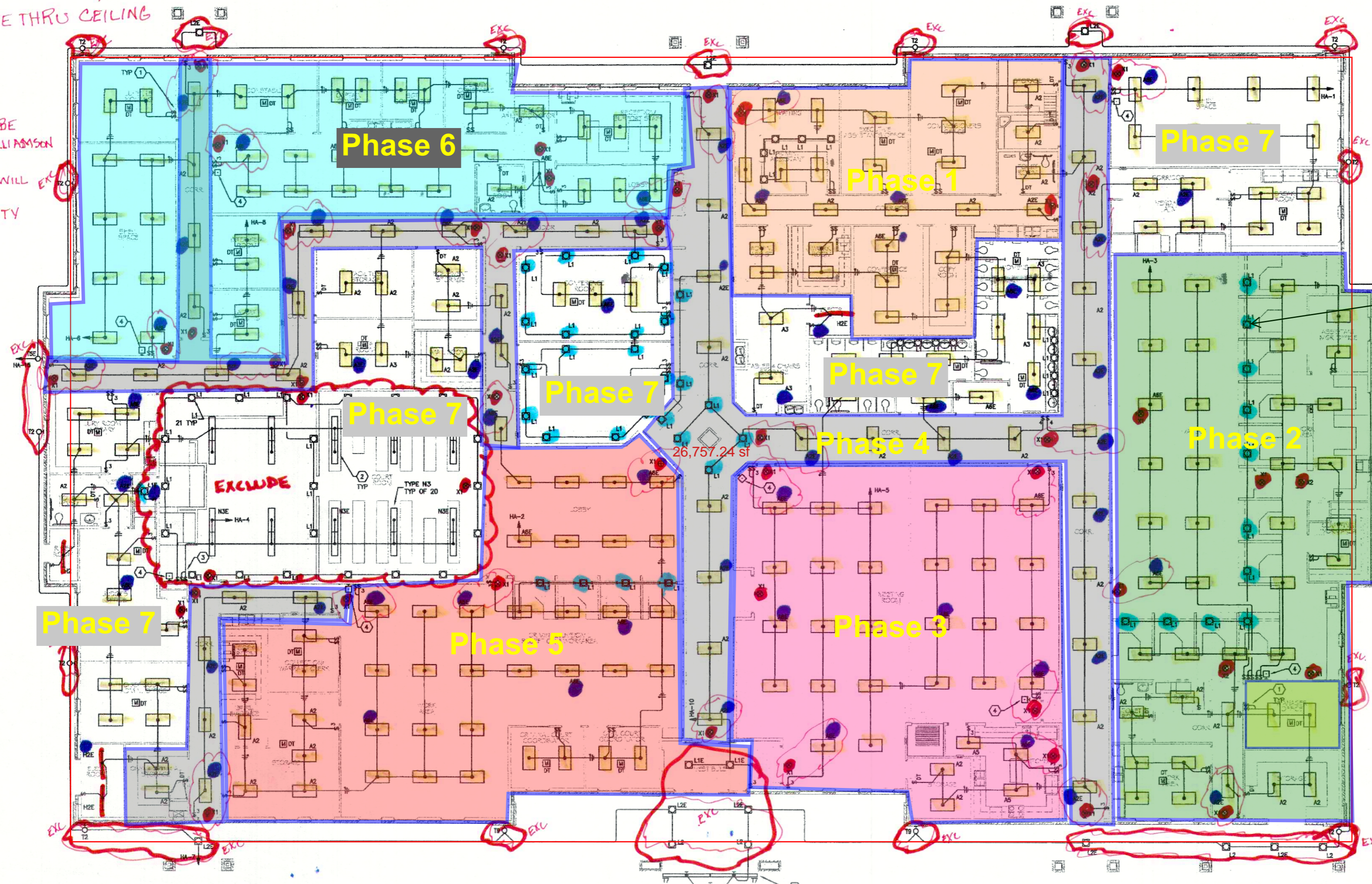
01 FLOOR PLAN - LIGHTING SCALE: 1/8" = 1'-0"
