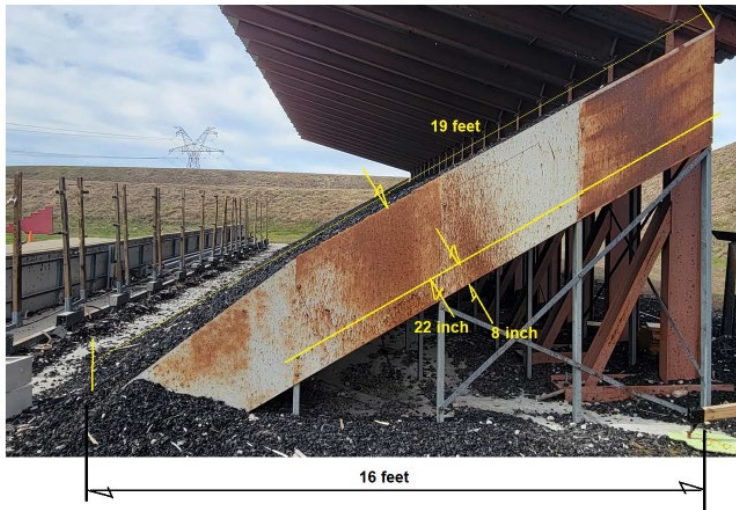
TYPICAL SIDE PROFILE FOR BOTH THE 50 YARD AND 200 YARD RANGE
