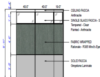
Elevation C
