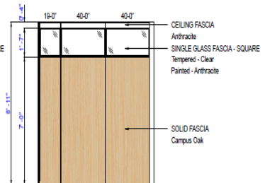
Elevation D
