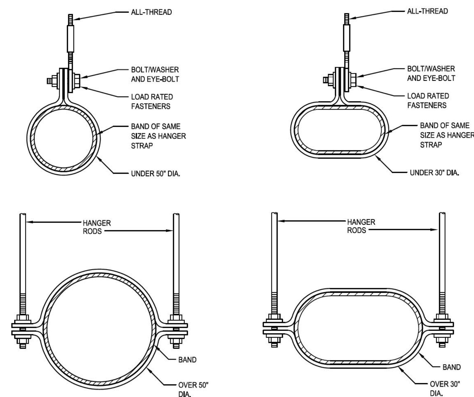
4 EXPOSED DUCT HANGER DETAIL
