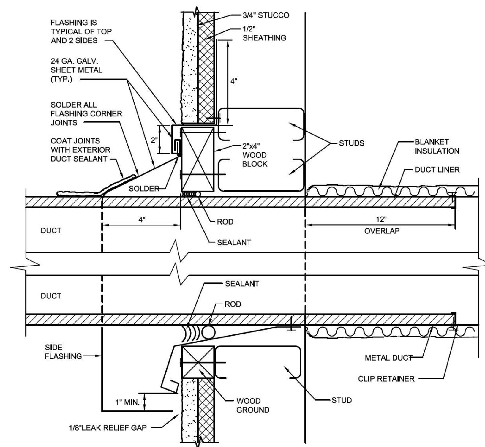
2 DUCT PENETRATION OF WALL ME501 NOT TO SCALE
