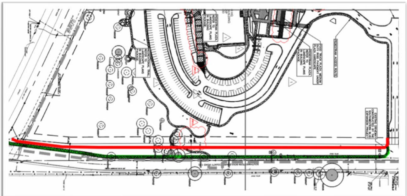
Image 1. Depiction of Sidewalk Modification. Current sidewalk location is shown in green, and proposed modification is shown in red.
