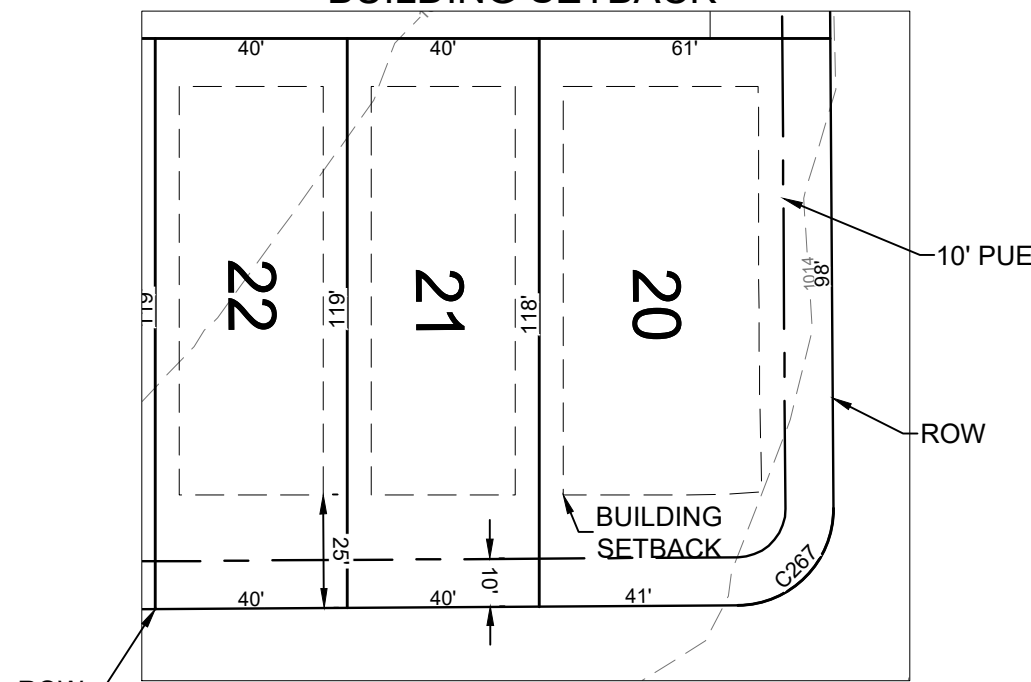
TYPICAL BUILDING SETBACK
