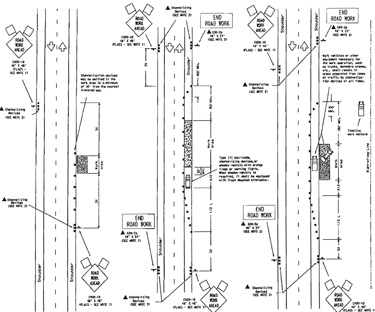
TCP (1-1c) Work Vehicles on Shoulder
