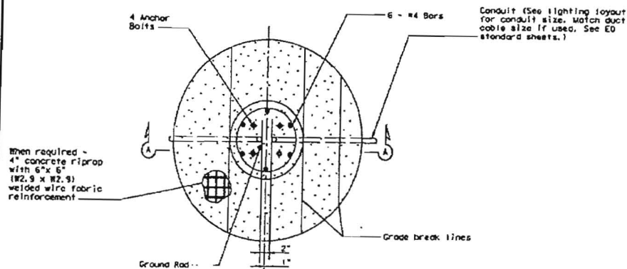
FOUNDATION DETAIL
