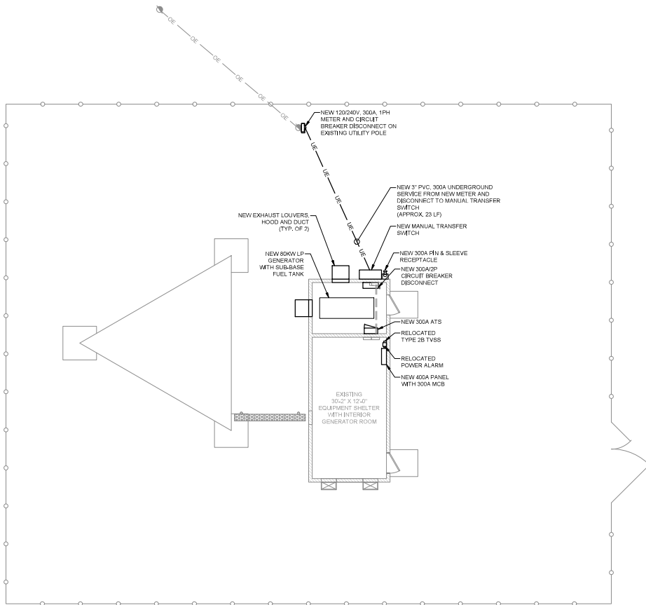
1 NEW UTILITY PLAN SCALE: 1" = 10'
