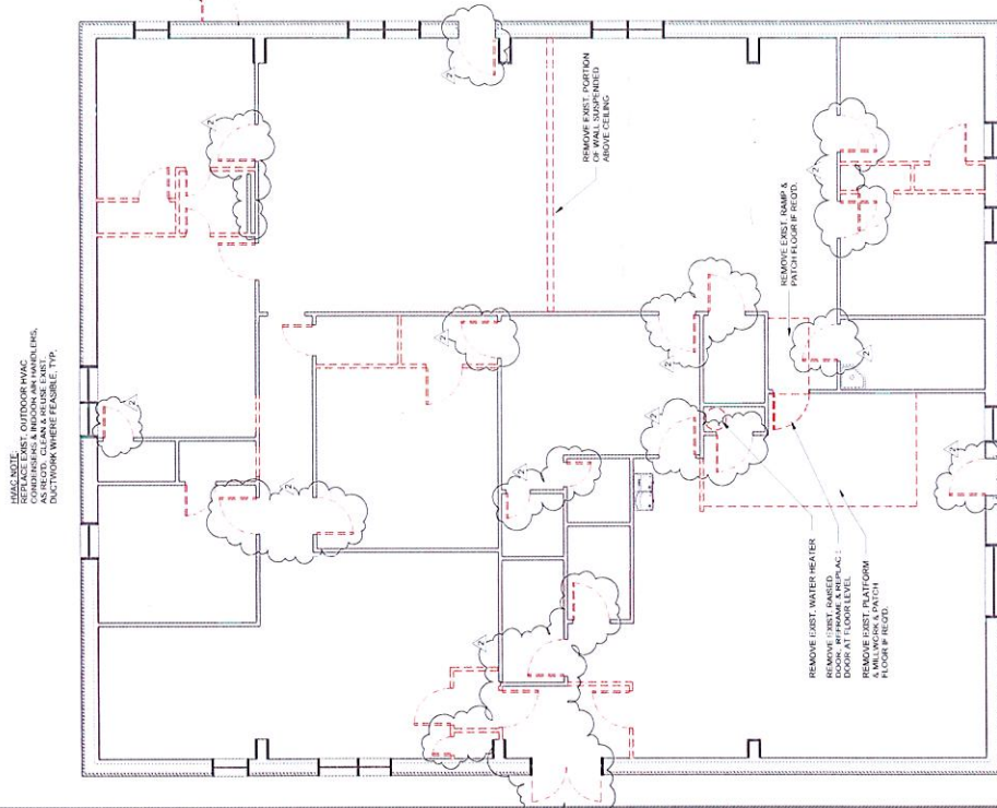
1 DEMOLITION PLAN 3/16" = 1'-0"
