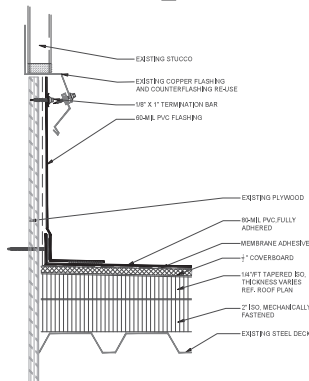
2 SOUTH ROOF EJ SCALE: 3/4"=1'-0"
