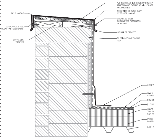
1 PARAPET WALL COPING CAP SCALE: 3/4"=1'-0"
