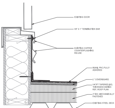
4 DOOR THRESHOLD SCALE: NTS
