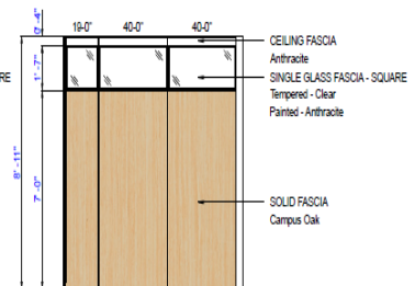
Elevation D
