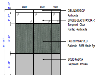
Elevation C
