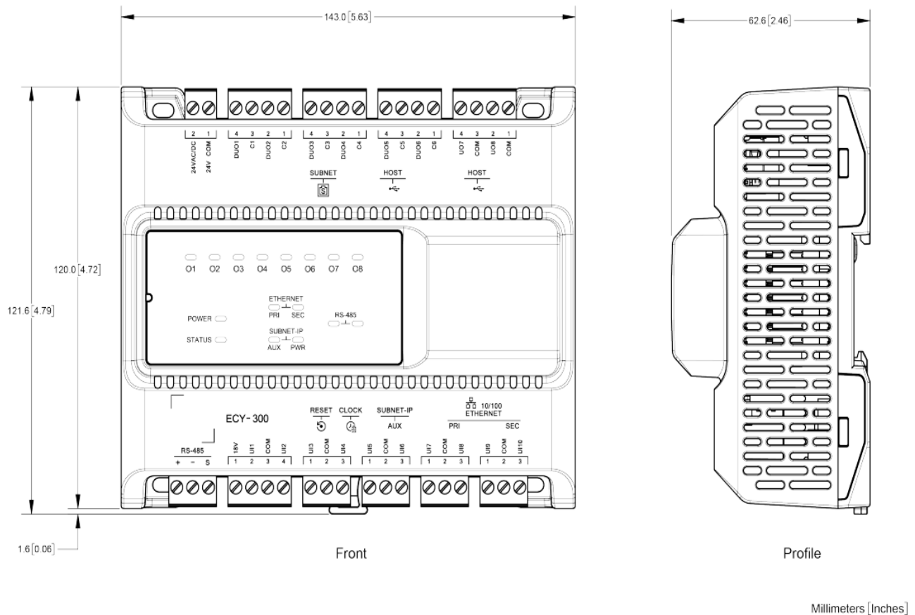
Figure 2. Controllers not equipped with an operator interface
