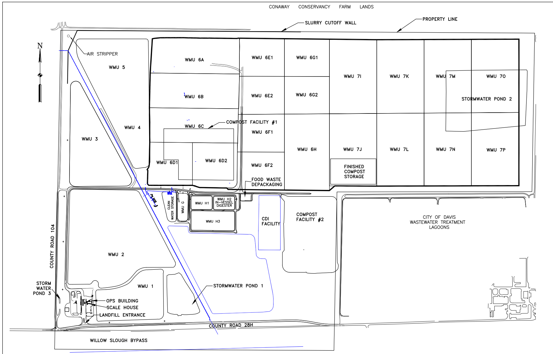
Figure 2 Existing Site Plan
