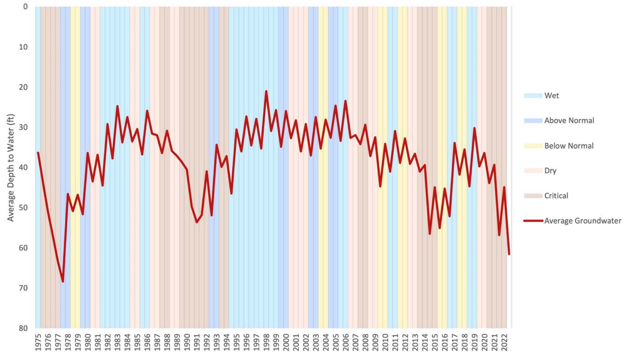
Yolo Subbasin Average Groundwater Representative Wells - Depth by Season (62 Wells)
