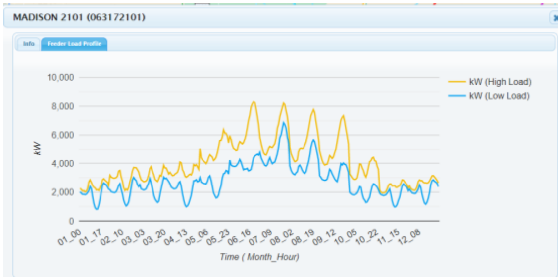
Figure 5: Madison 2101 Distribution Load Profile
