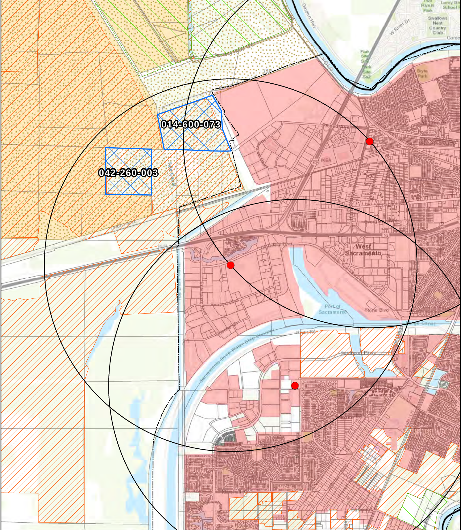
Figure D-13 Gibson Solar Farm - West Sacramento Substation
