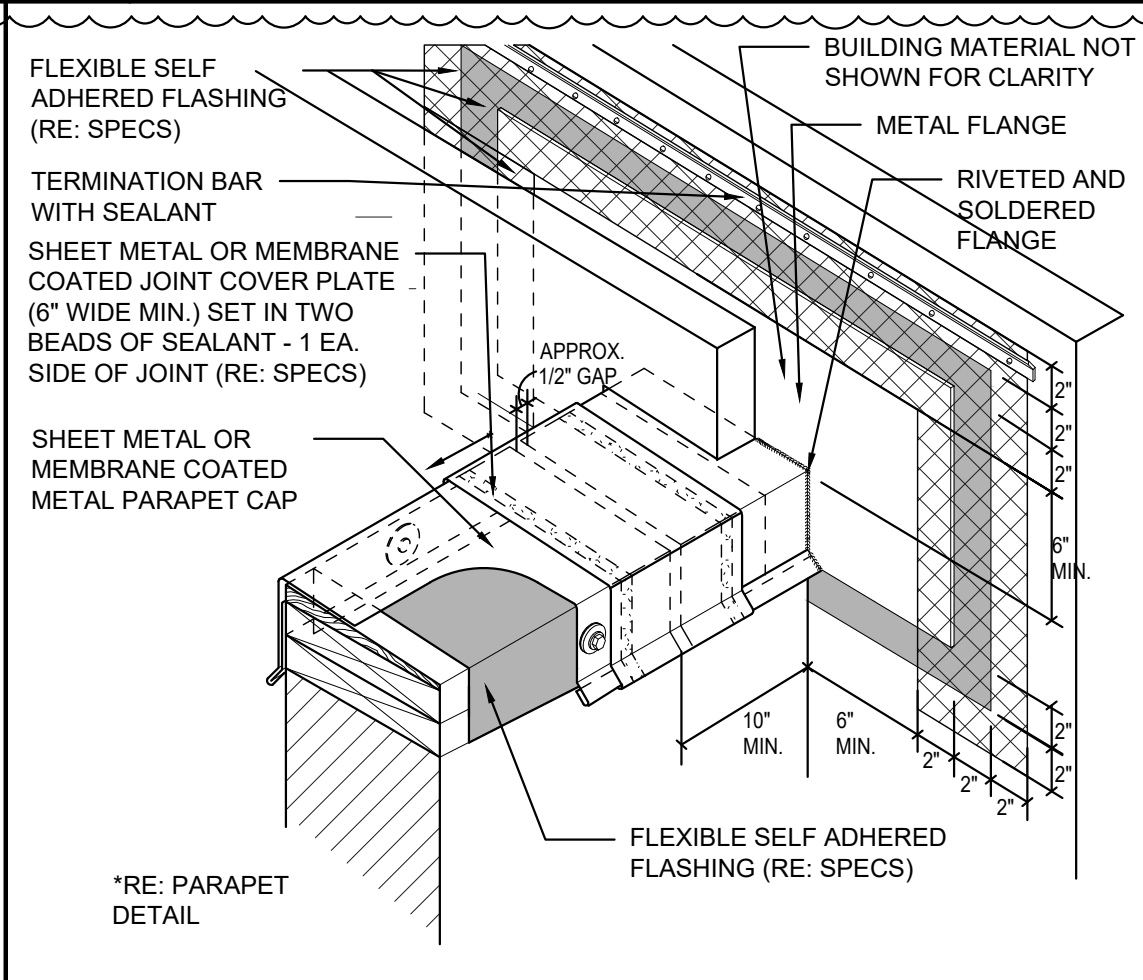
3 PARAPET SADDLE NOT TO SCALE
