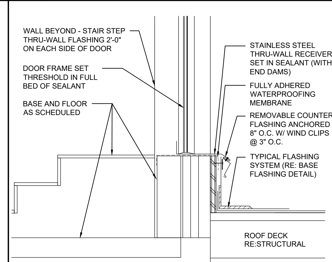
6 ROOF ACCESS DOOR NOT TO SCALE
