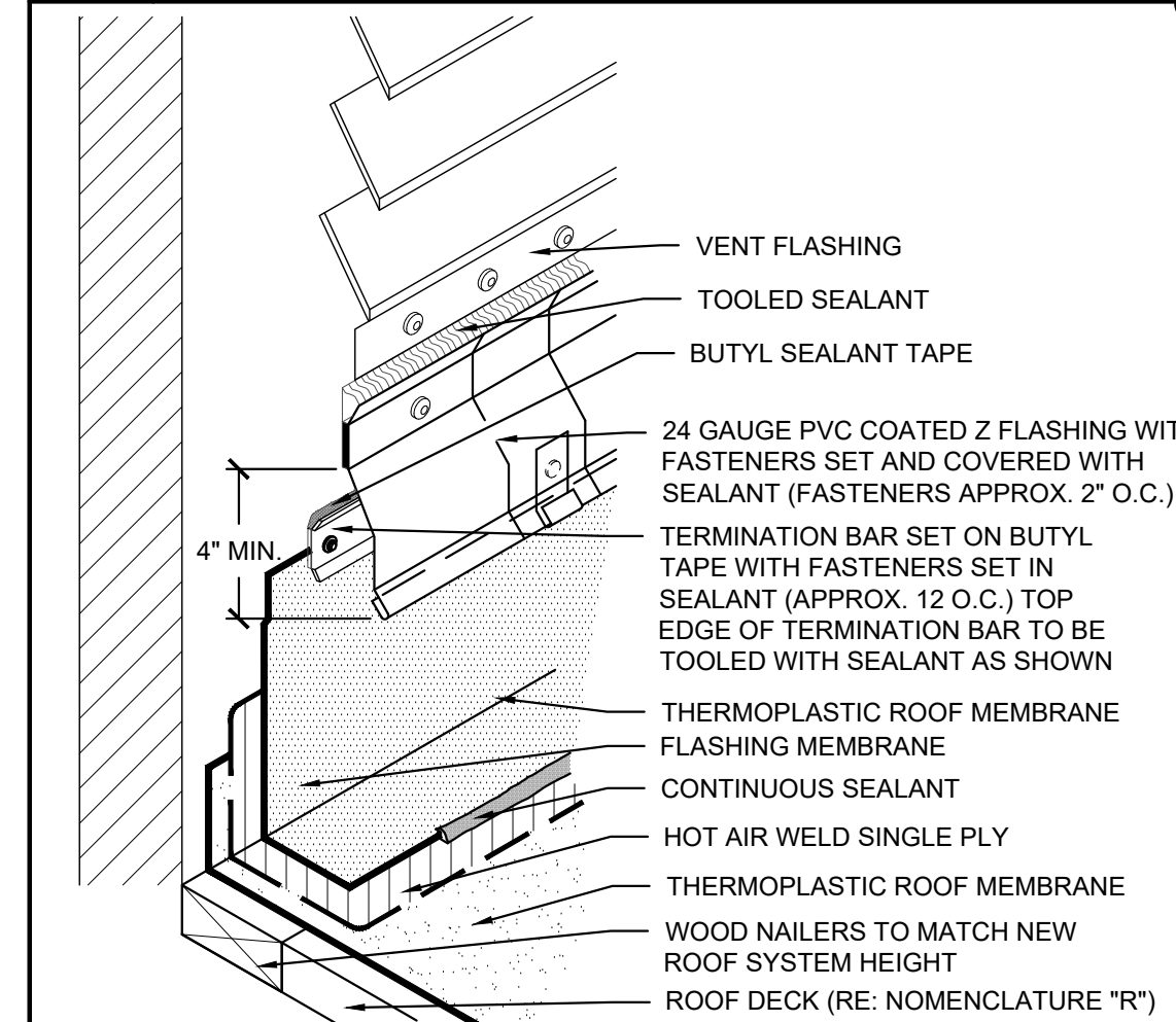
4 VENT FLASHING NOT TO SCALE
