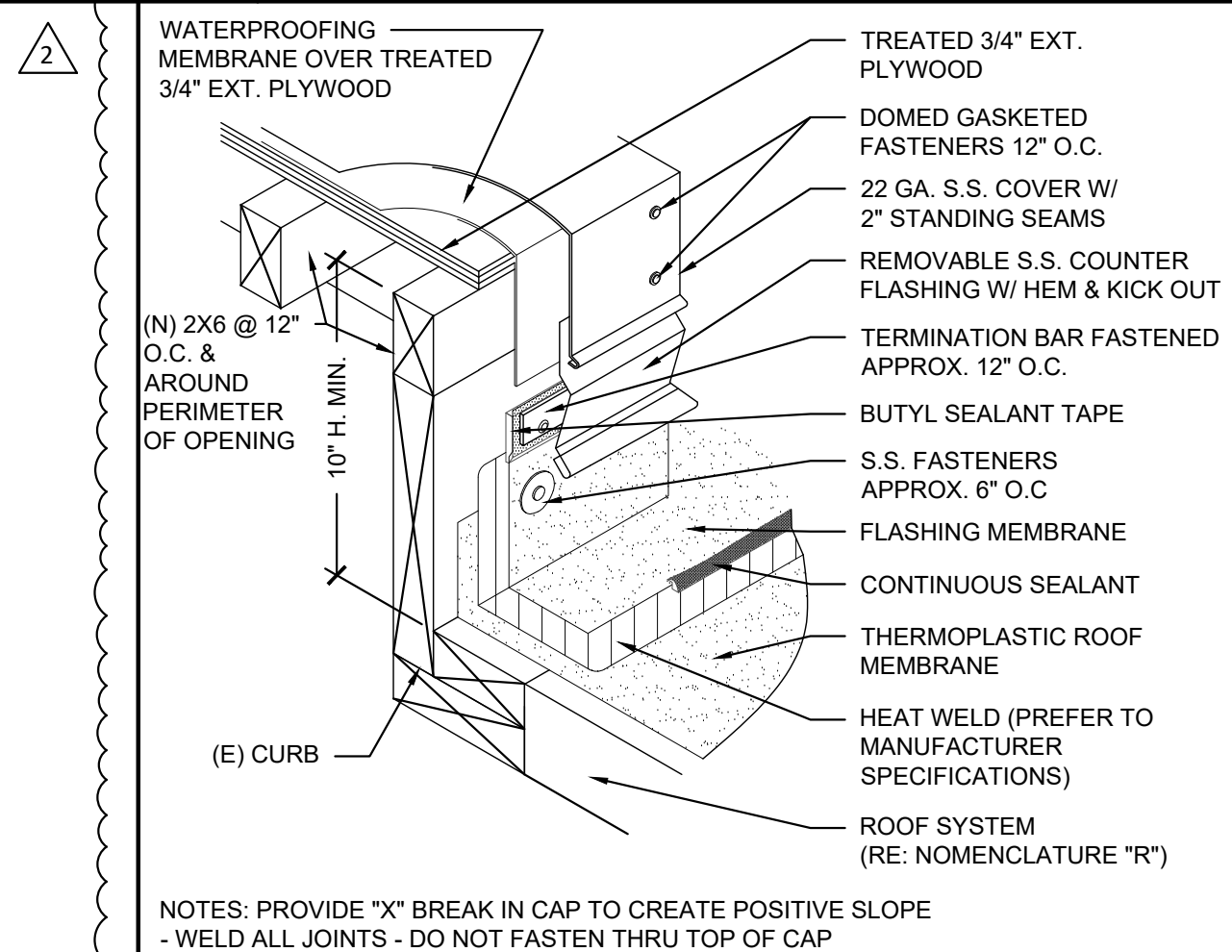
8 CAP EXISTING CURB NOT TO SCALE
