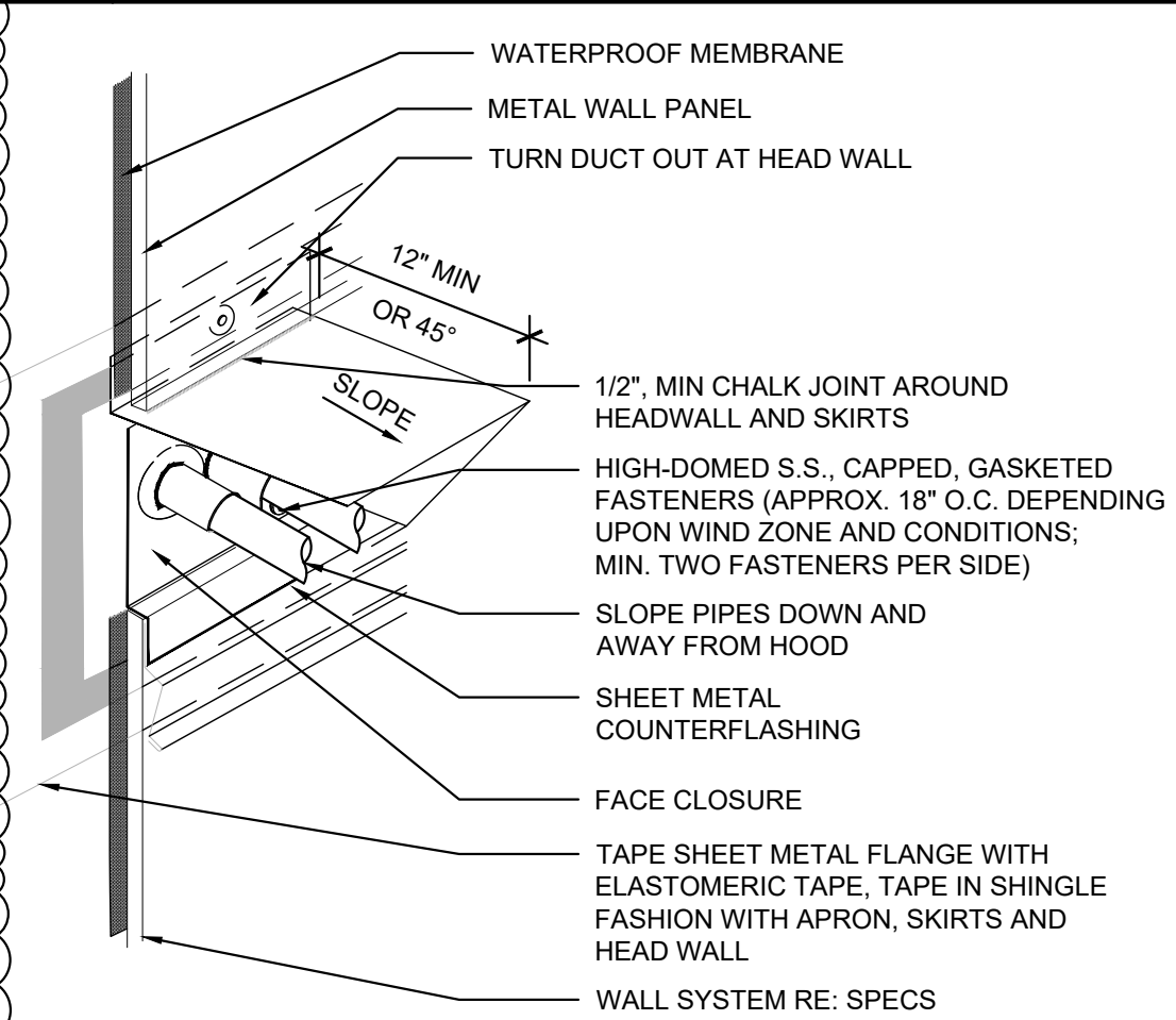
7 HOOD AT WALL PENETRATION
