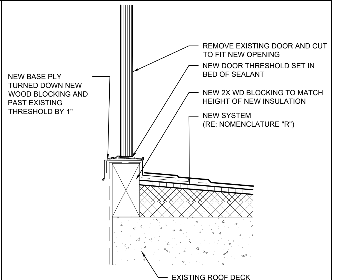
5 DOOR THRESHOLD FLASHING NOT TO SCALE
